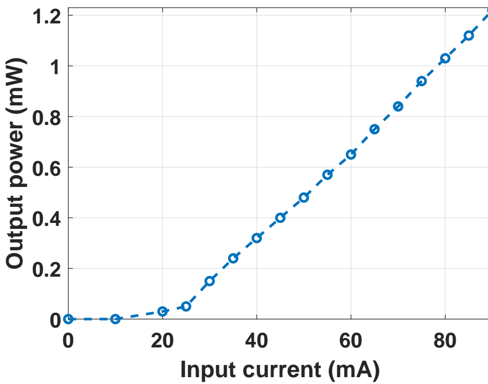
Laser characteristics
