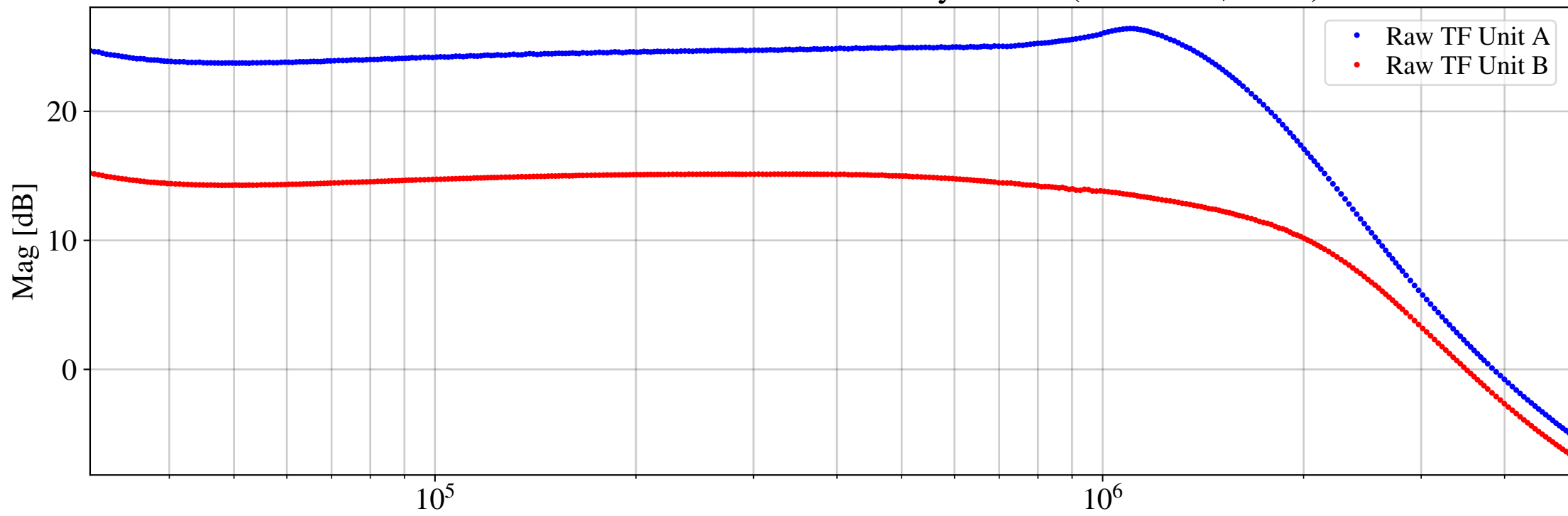
Raw transfer functions of WOPO Homodyne PDs (March 27, 2019)
