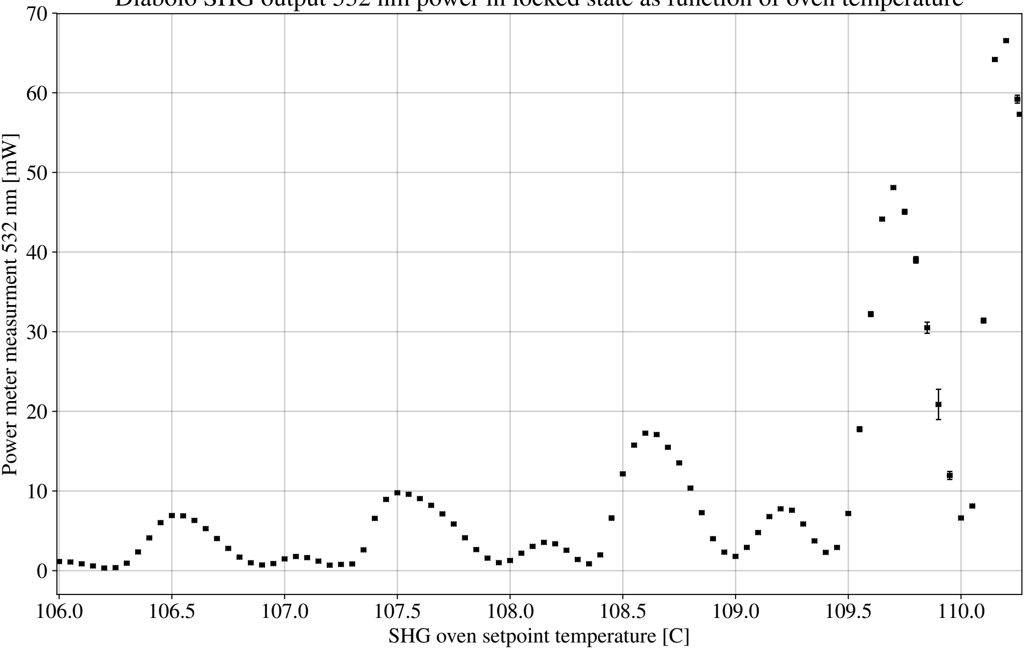
Diabolo SHG output 532 nm power in locked state as function of oven temperature
