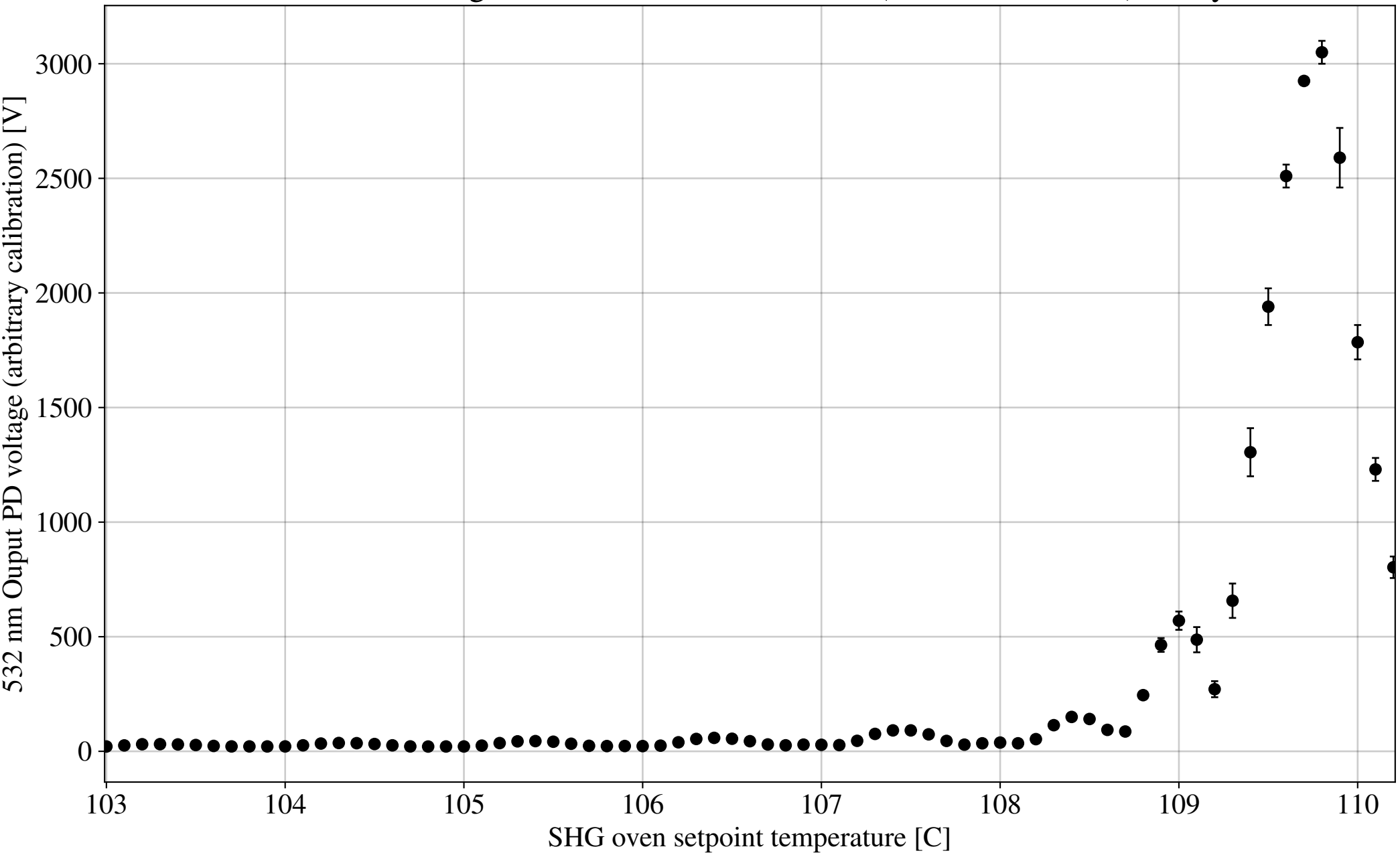
Phase matching curve for Diabolo SHG LN (in fast scan mode) cavity
