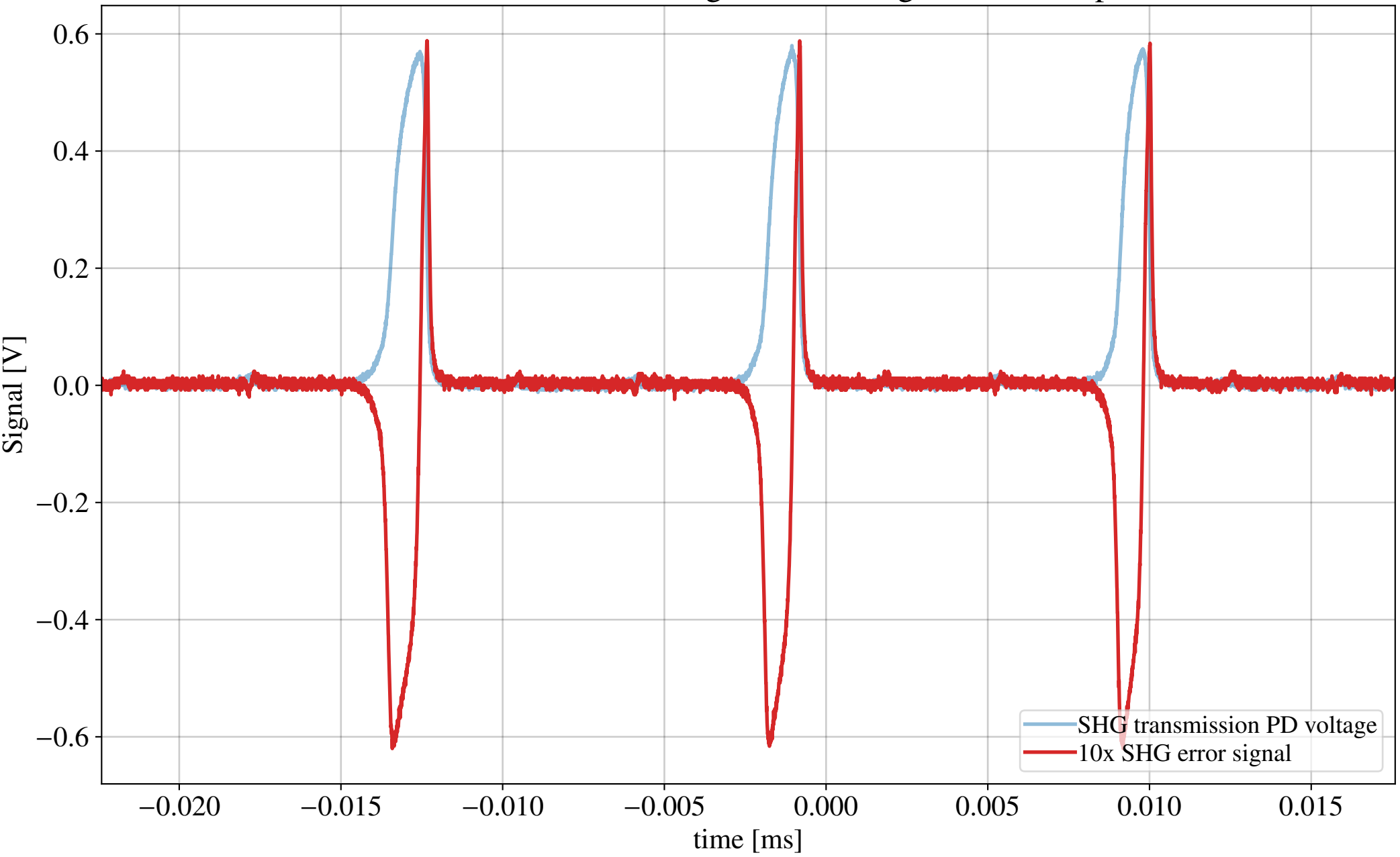
SHG Transmission Peaks And Error Signal After Alignment Tuneup - Dec 04, 2018
