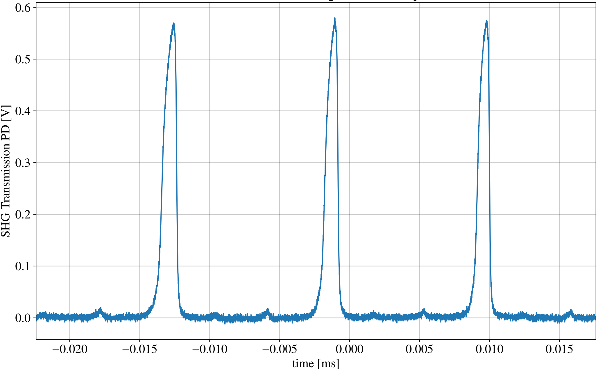
SHG Transmission Peaks After Alignment Tuneup - Dec 04, 2018
