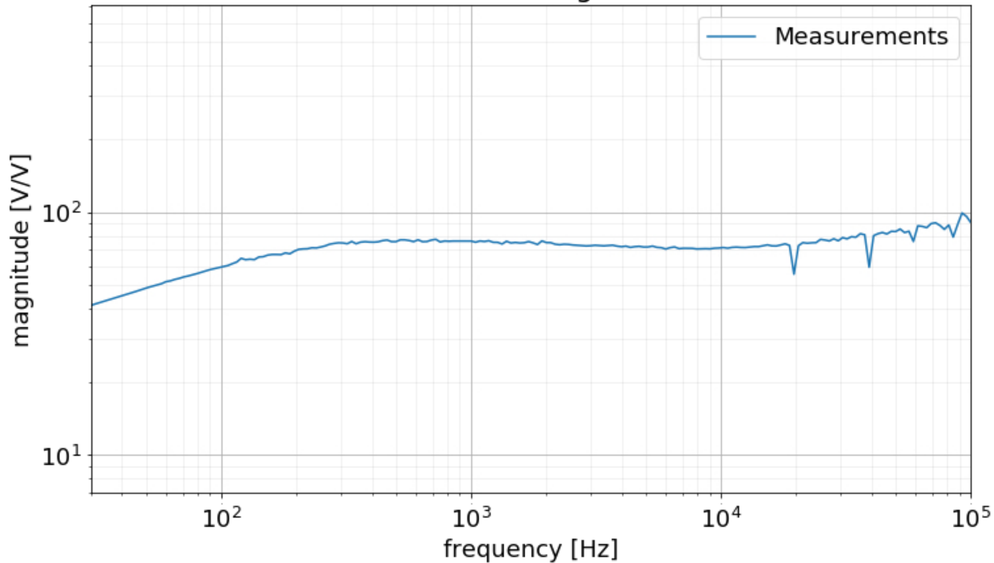
BHD Transfer Function - Aug 07 2018 - 14:37:28
