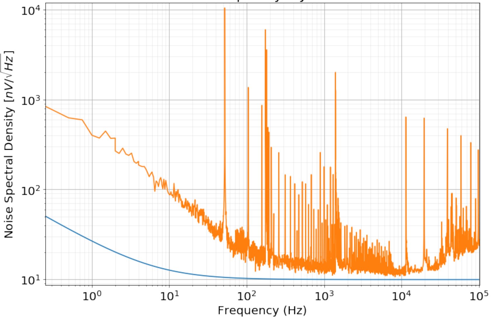
Electronic Noise vs. Frequency - Jul-20-2018 - 12:11:34
