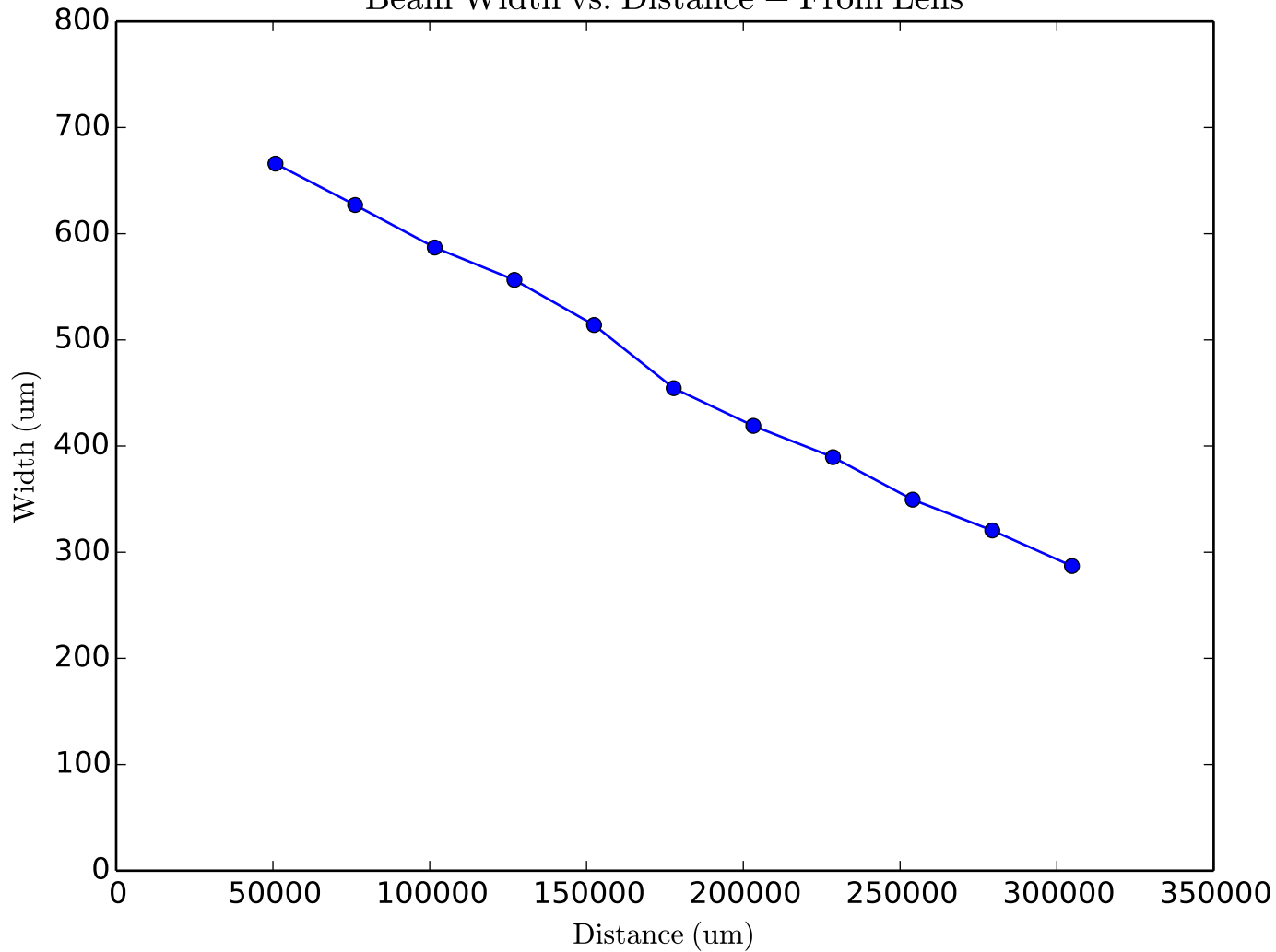
Beam Width vs. Distance – From Lens
