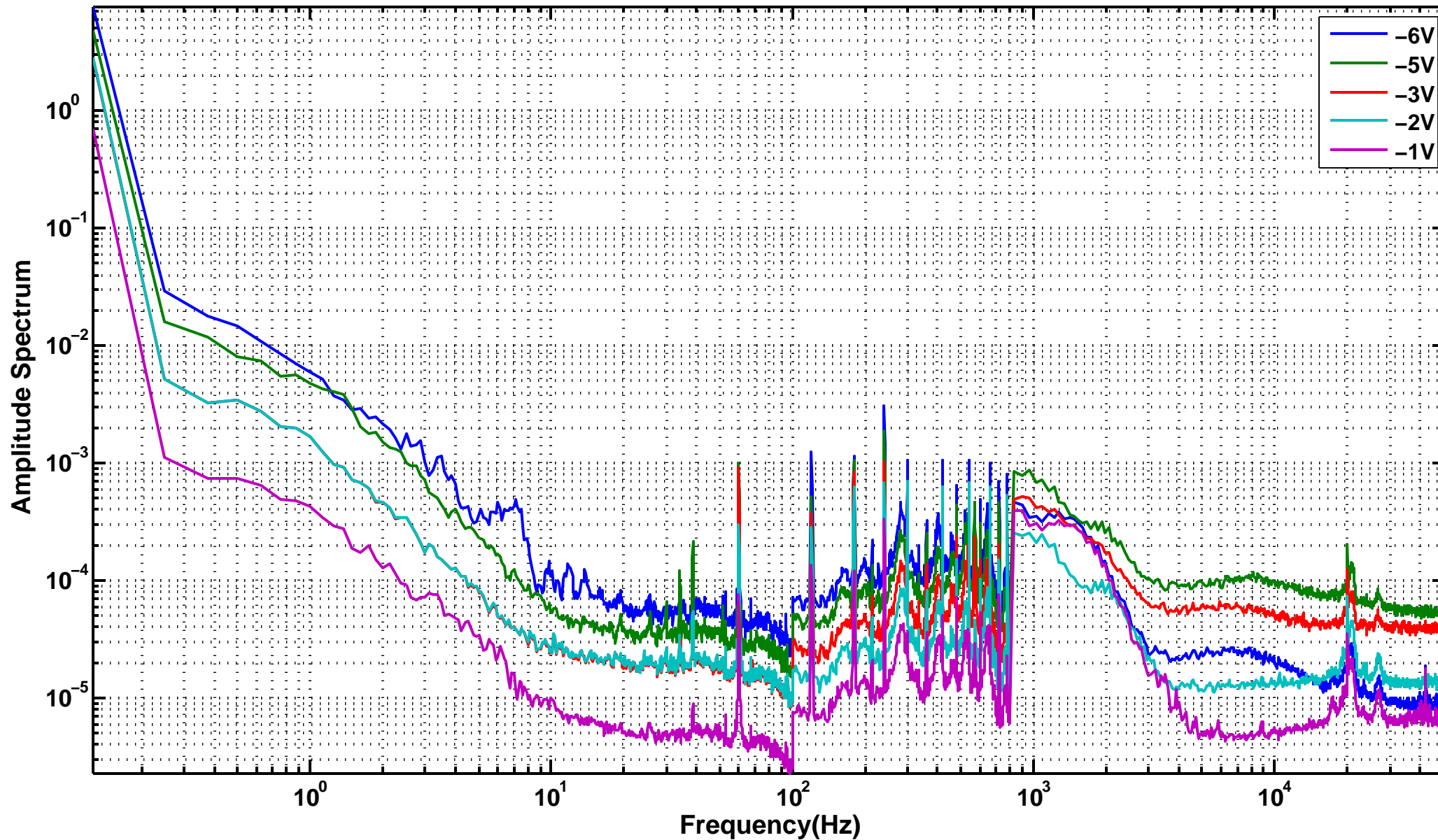
Free Running Laser noise for different DC bias points( This is set by the intensity of the laser)
