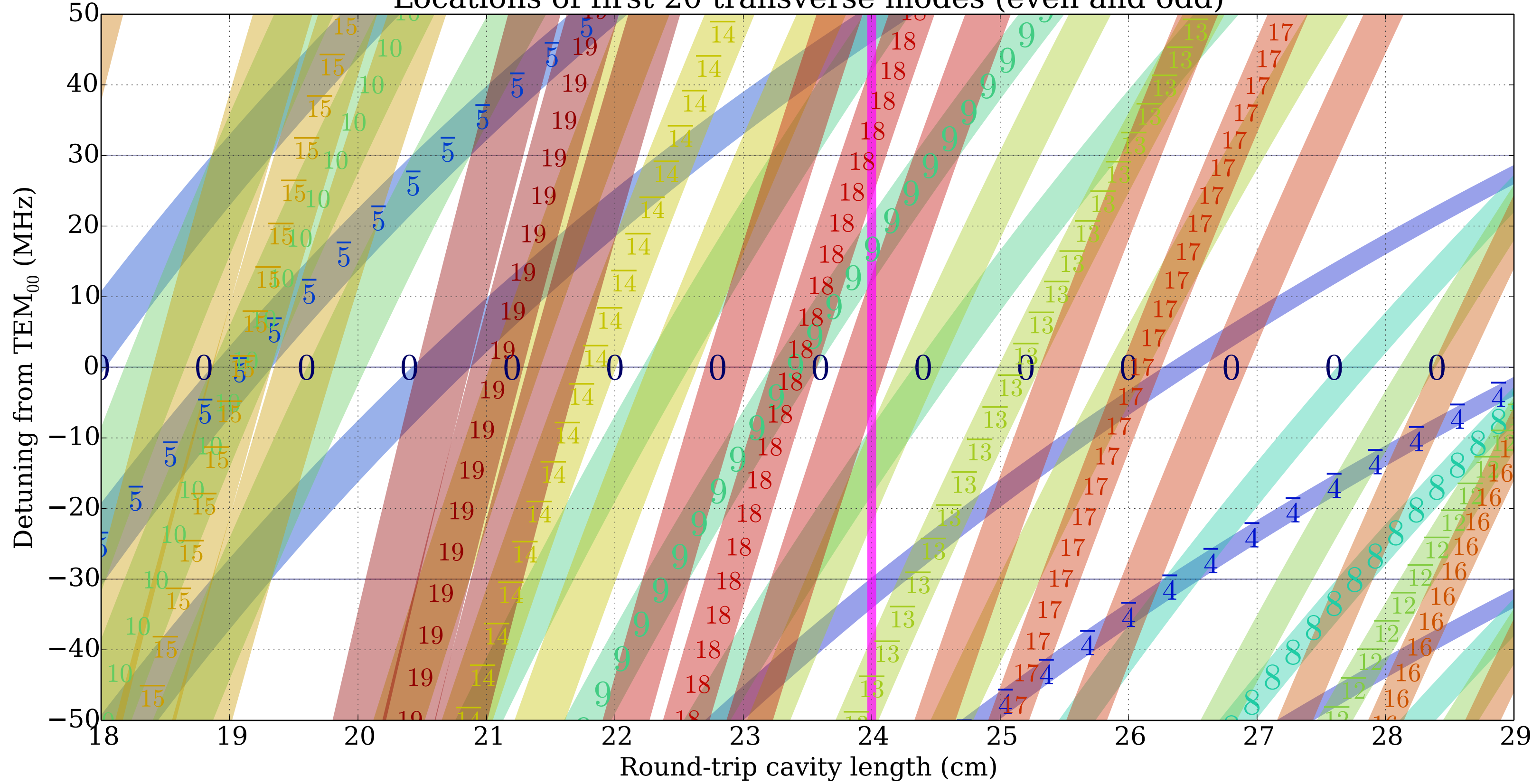
Locations of first 20 transverse modes (even and odd)
