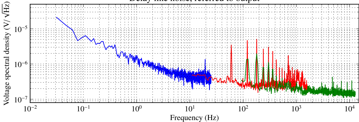
Delay line noise, referred to beat frequency
