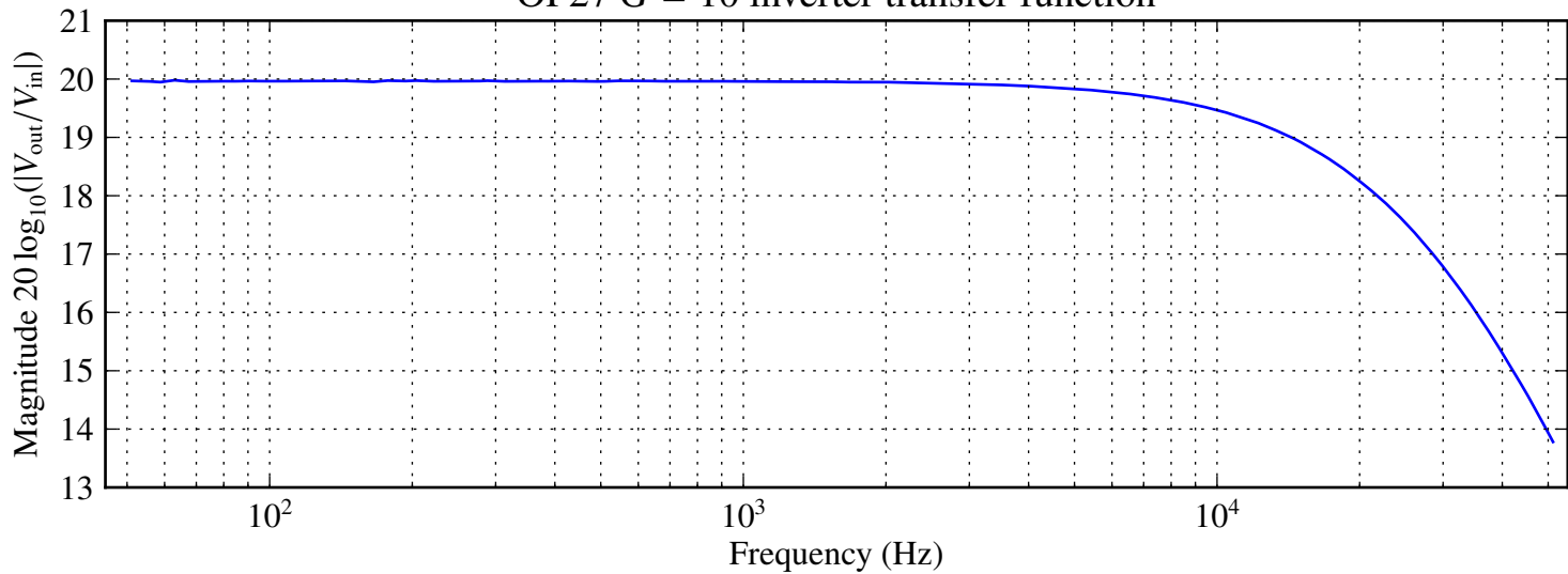
OP27 G = 10 inverter transfer function
