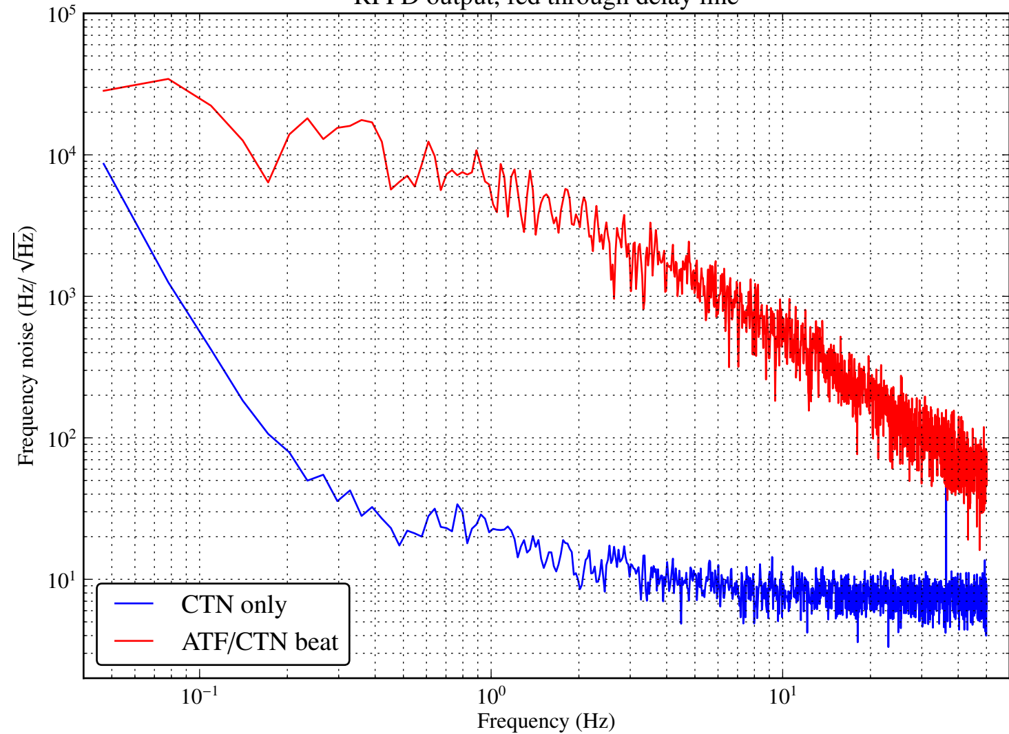
RFPD output, fed through delay line
