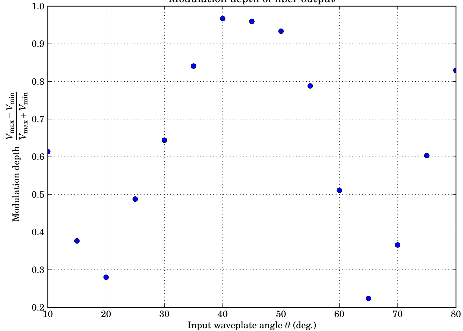
Modulation depth of fiber output
