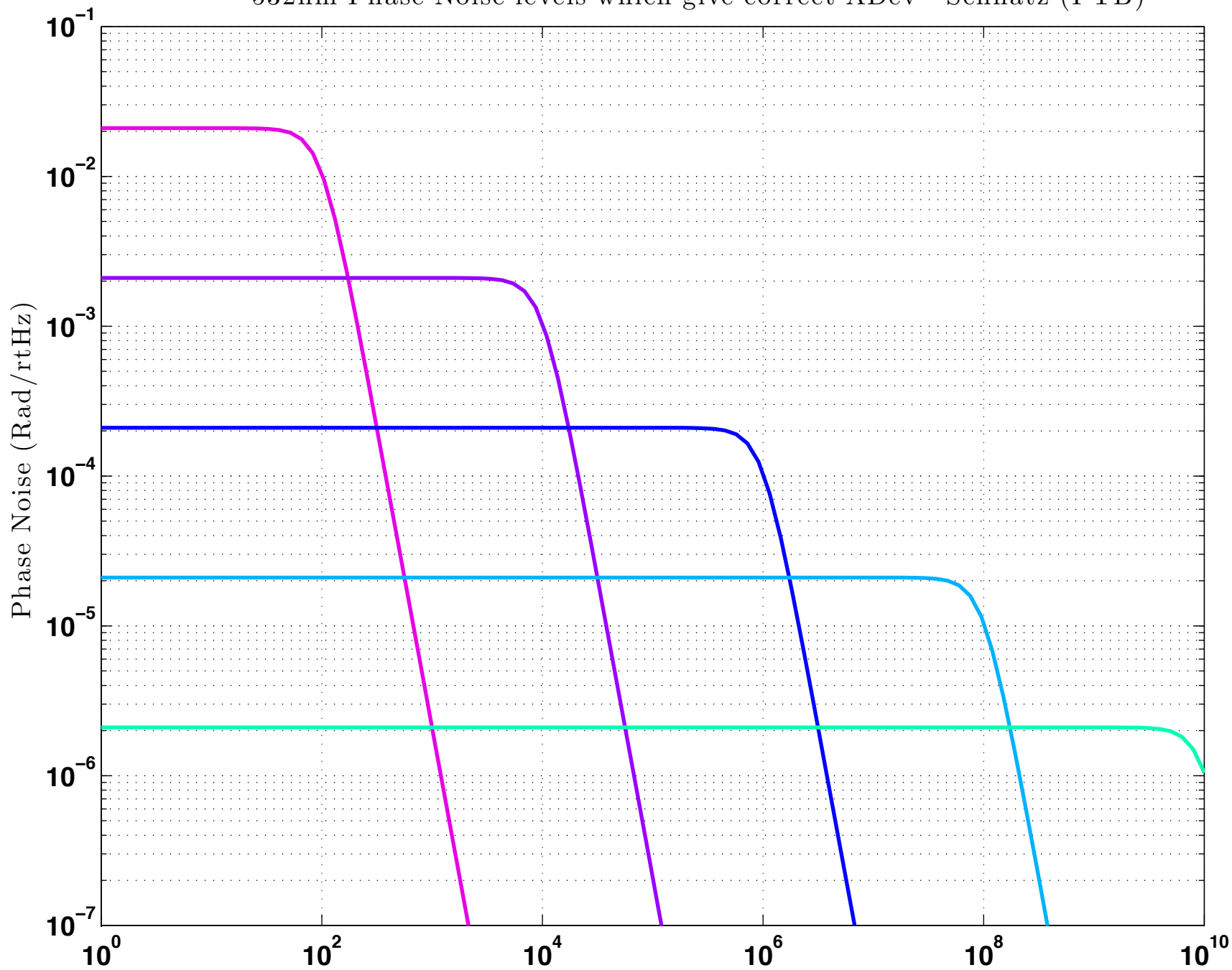
532nm Phase Noise levels which give correct ADev - Schnatz (PTB)
