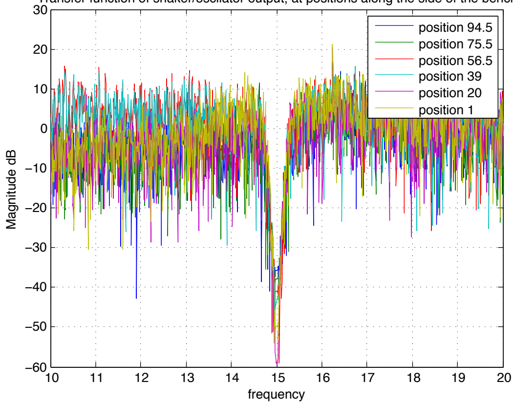
Transfer function of shaker/oscillator output, at positions along the side of the bench
