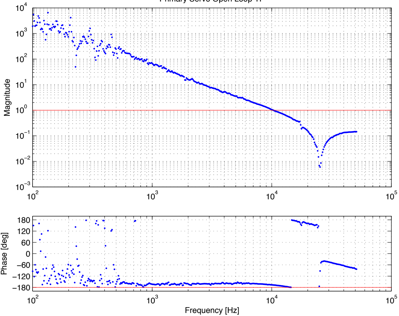
Primary Servo Open Loop TF
