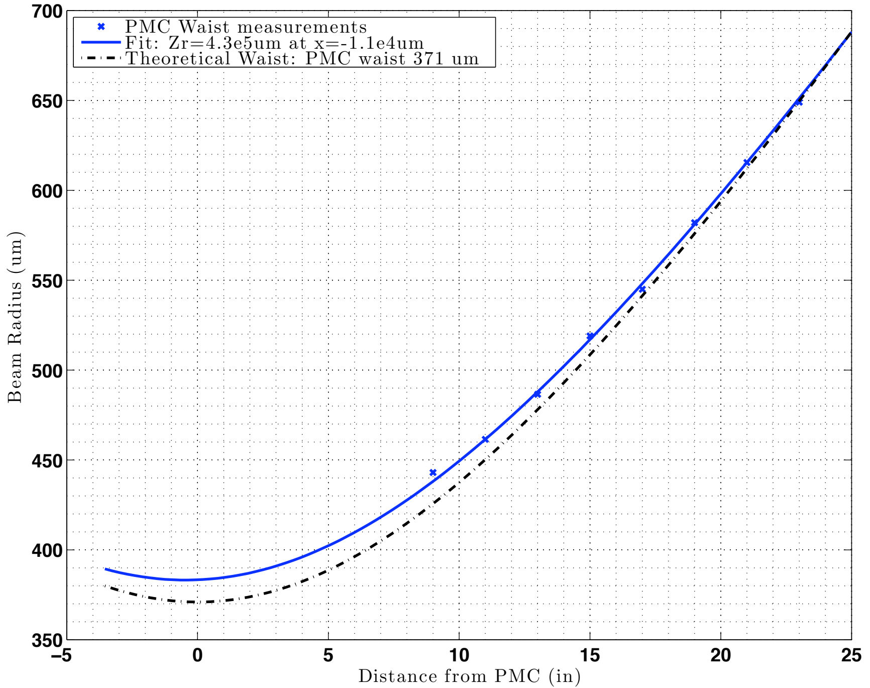
PMC Transmission Beam Profile
