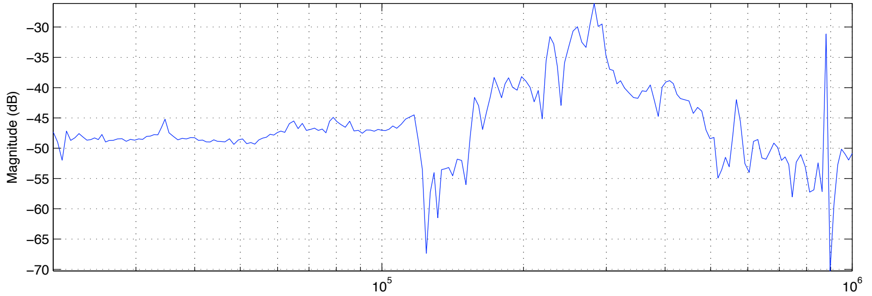
H1NPRO PZT FM Transfer Function
