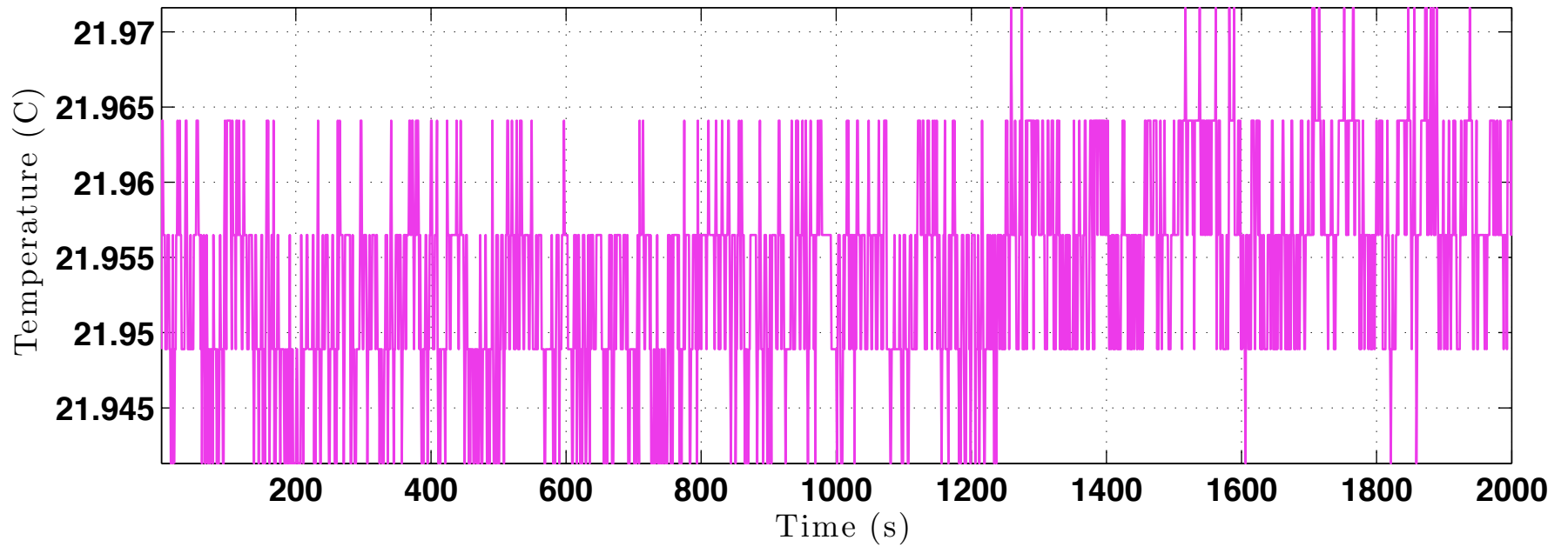
Open Loop Oven Temperature - No Box
