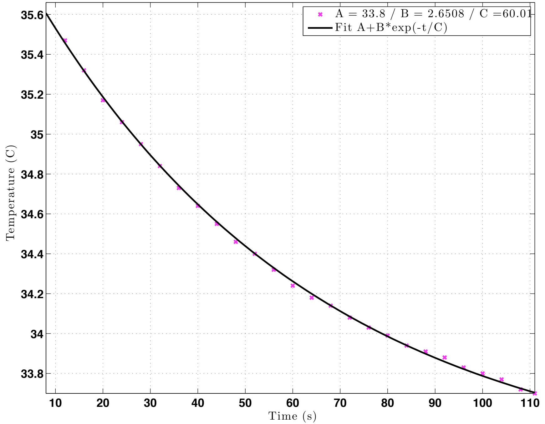
Cu Oven response to Current step 0.7A - > 0.58A
