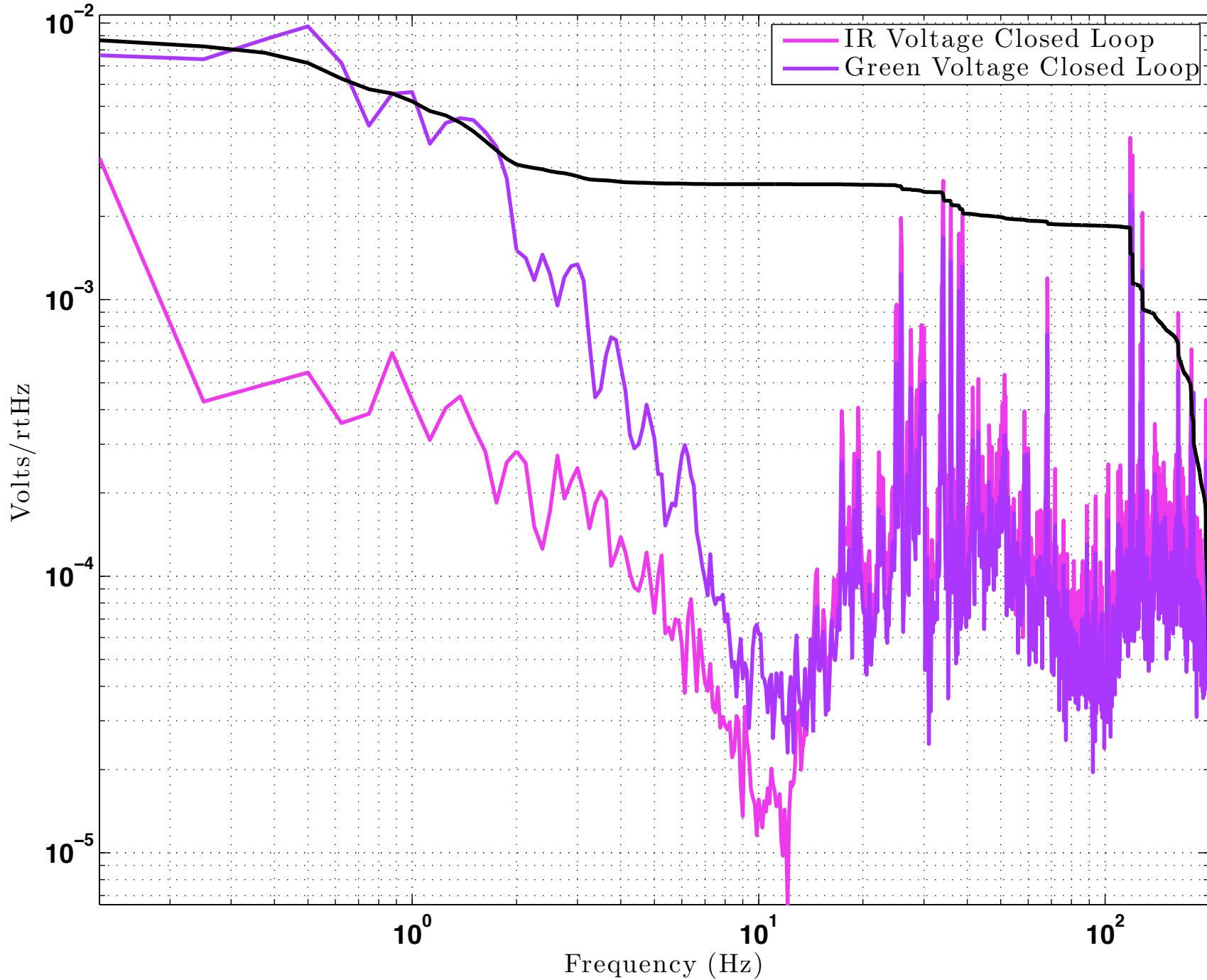
Voltage Noise of Mach Zehnder May 17 2010
