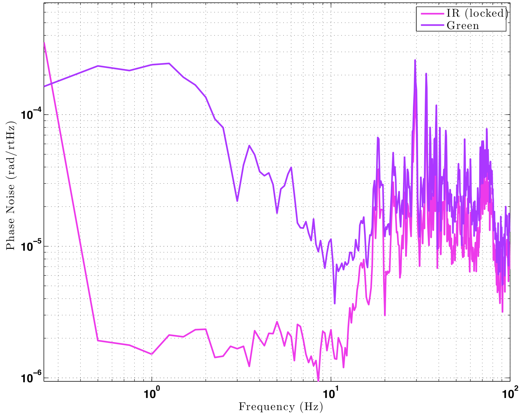
Locked Mach Zehnder Phase Noise
