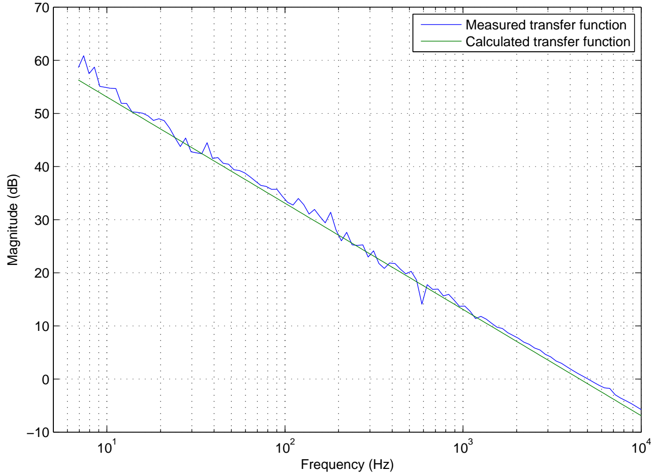
Fiber Stabilization Loop Transfer Function – magnitude only. 22nd Jan 2010
