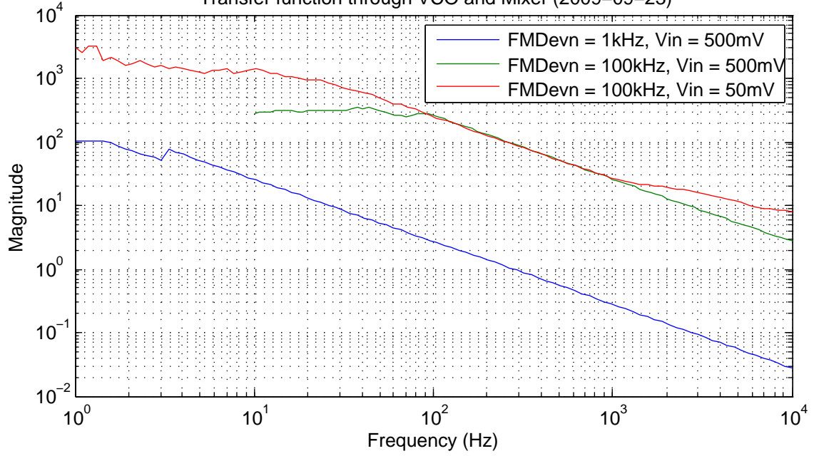
Transfer function through VCO and Mixer (2009-09-23)
