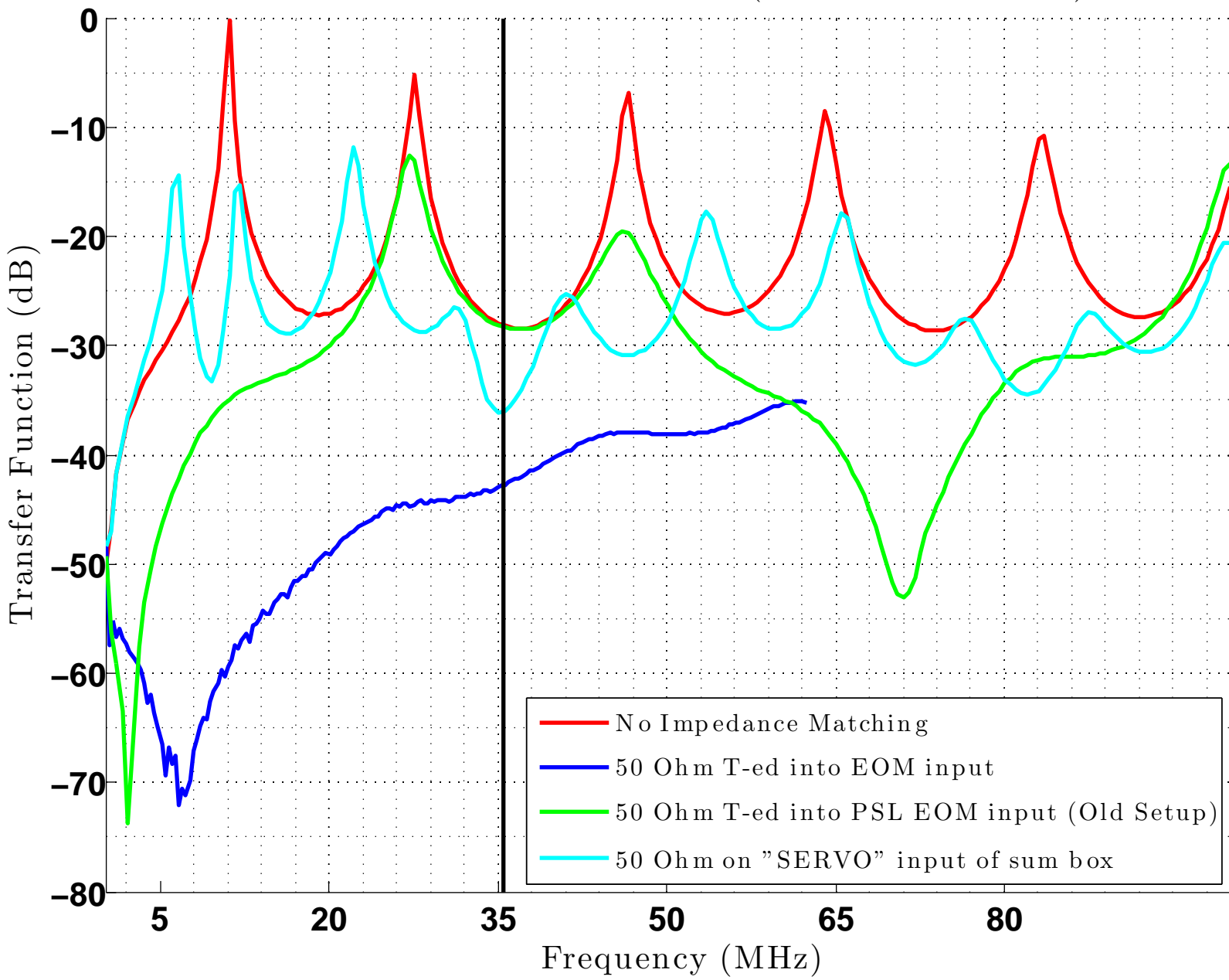
RF Reflection from EOM (Transfer Functions)
