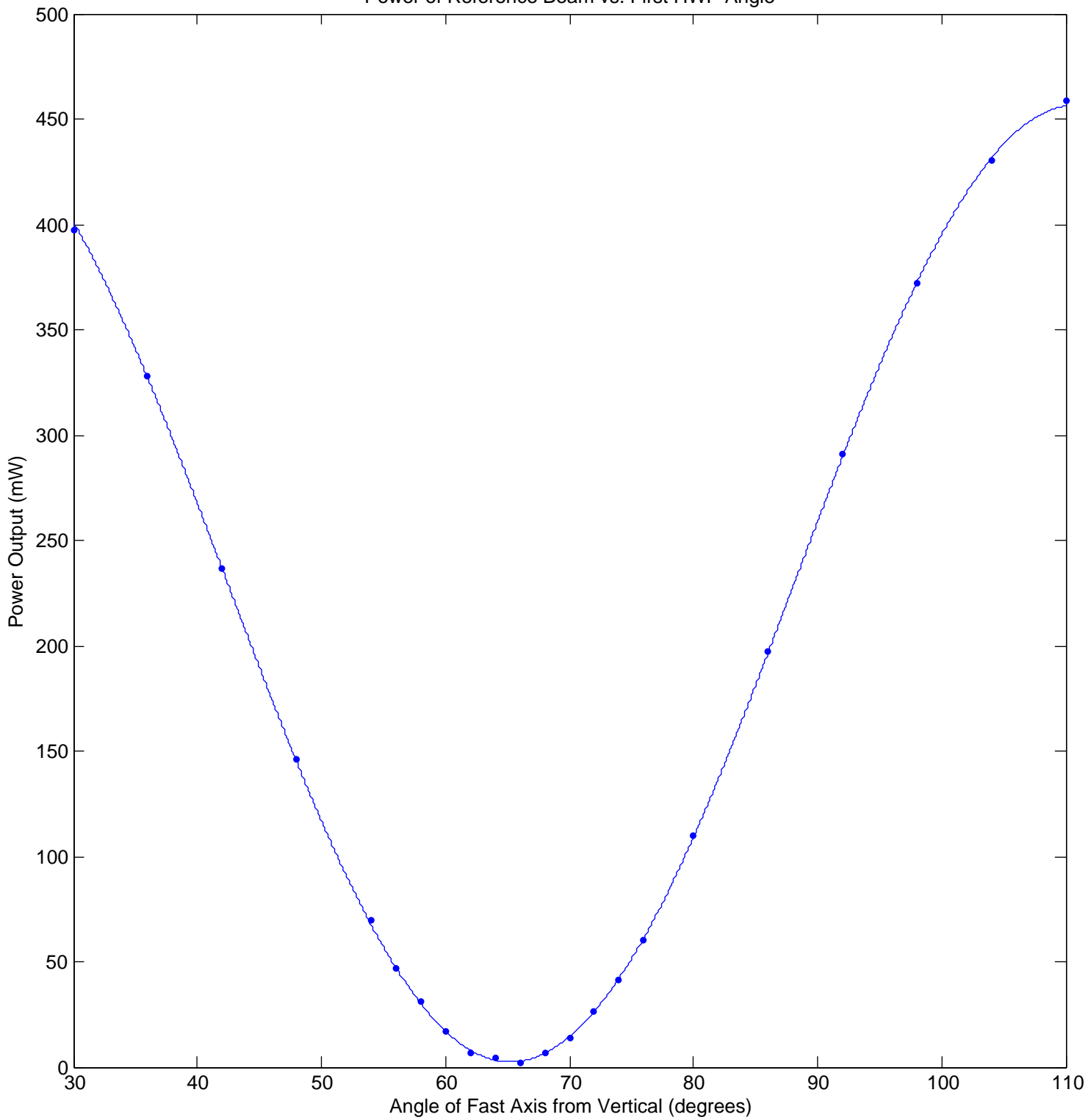
Power of Reference Beam vs. First HWP Angle
