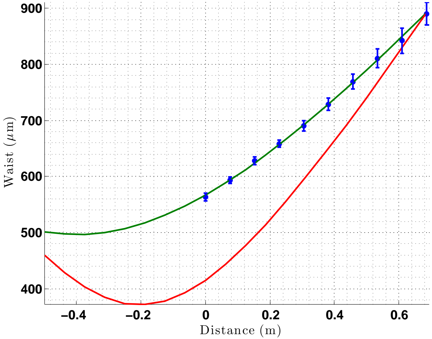
Beam Entering PMC and PMC Ideal Waist/Position
