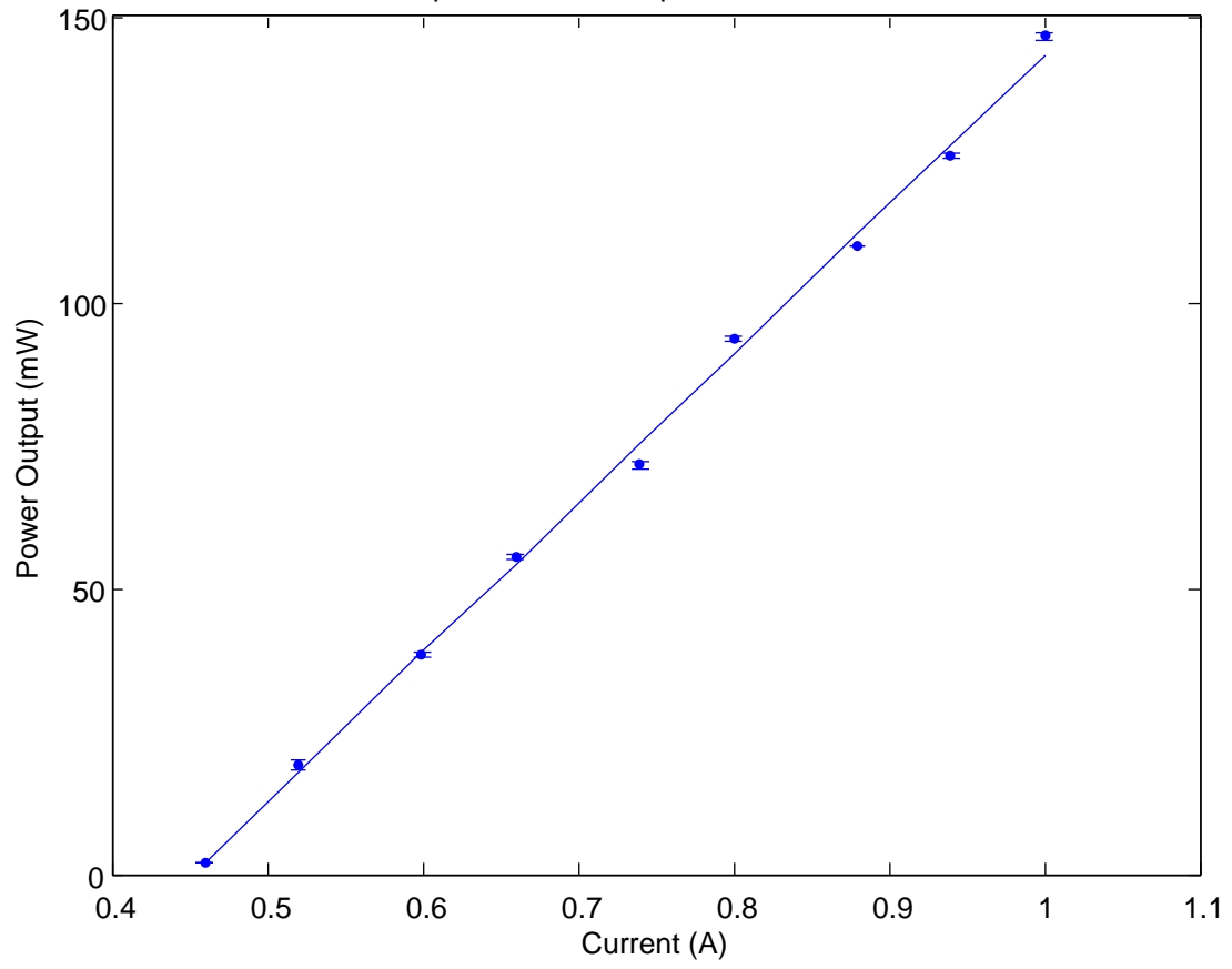
Power Output vs. Current Input of 495mW NPRO Laser
