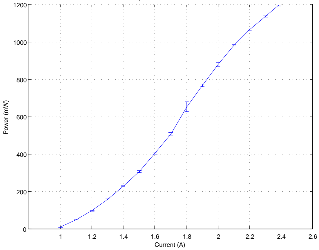
Power Output vs. Current for Nd-YAG Laser
