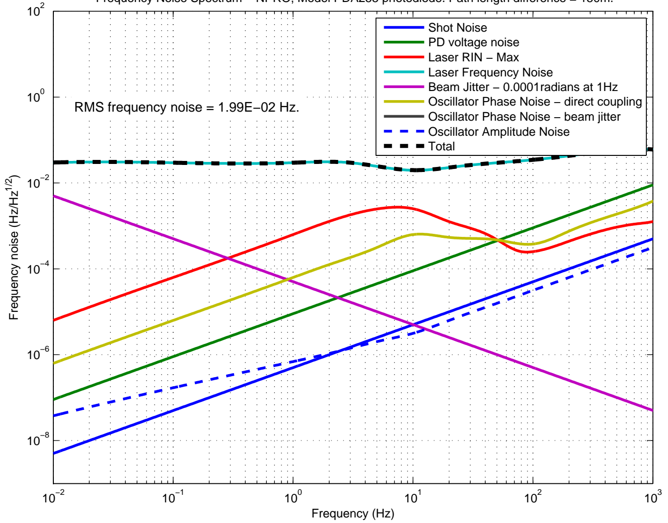
Frequency Noise Spectrum – NPRO, Model PDA255 photodiode. Path length difference = 150m.
