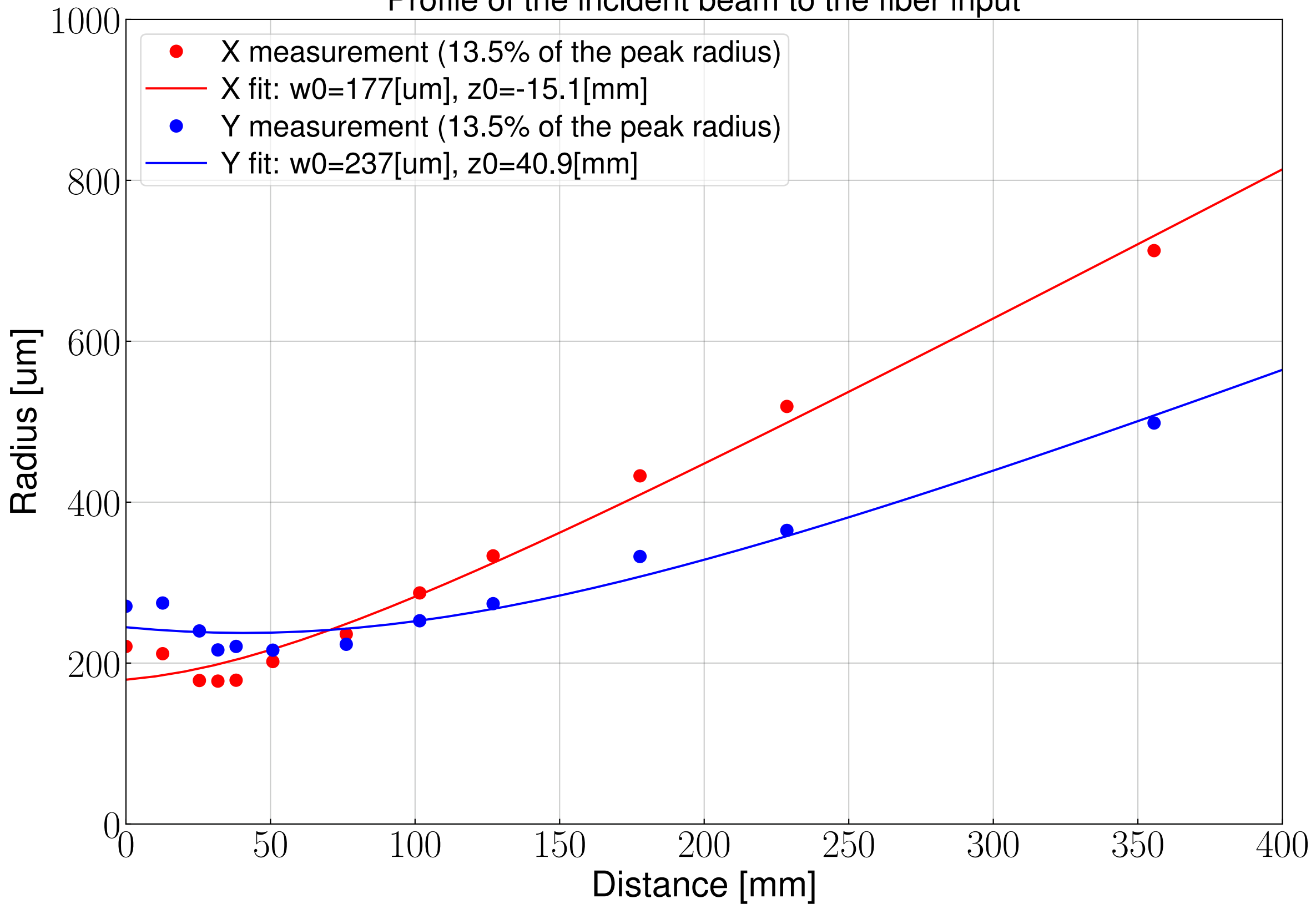
Profile of the incident beam to the fiber input
