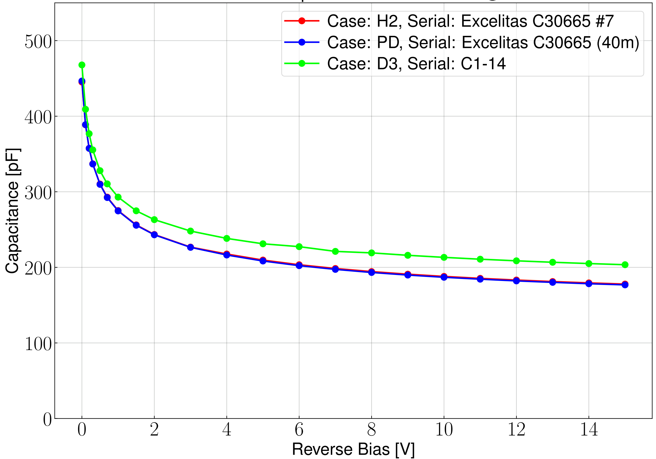
Excelitas C30665 capacitance measurement @100kHz
