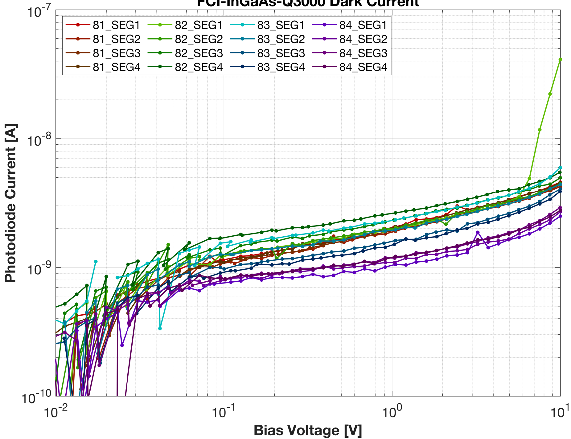
FCI-InGaAs-Q3000 Dark Current
