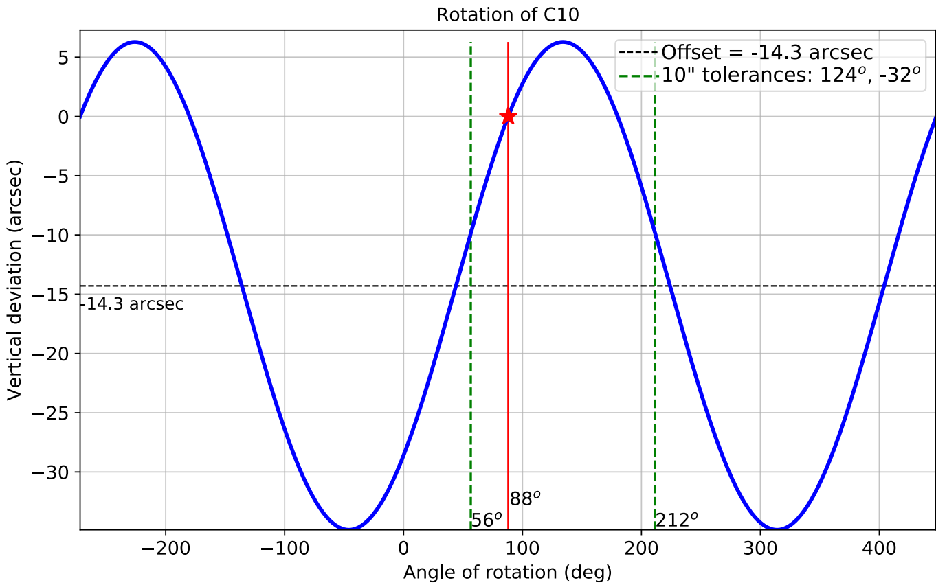
(Fig 1.1) C10 rotated by 88 deg + PZT12 at 0deg + M12
