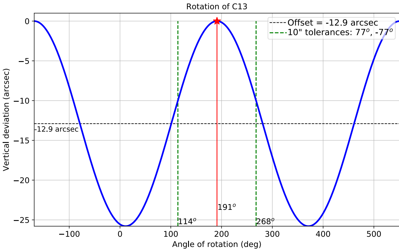
(Fig 1.2) C13 rotated by 191deg(-169deg) + PZT13 at 0deg + M14
