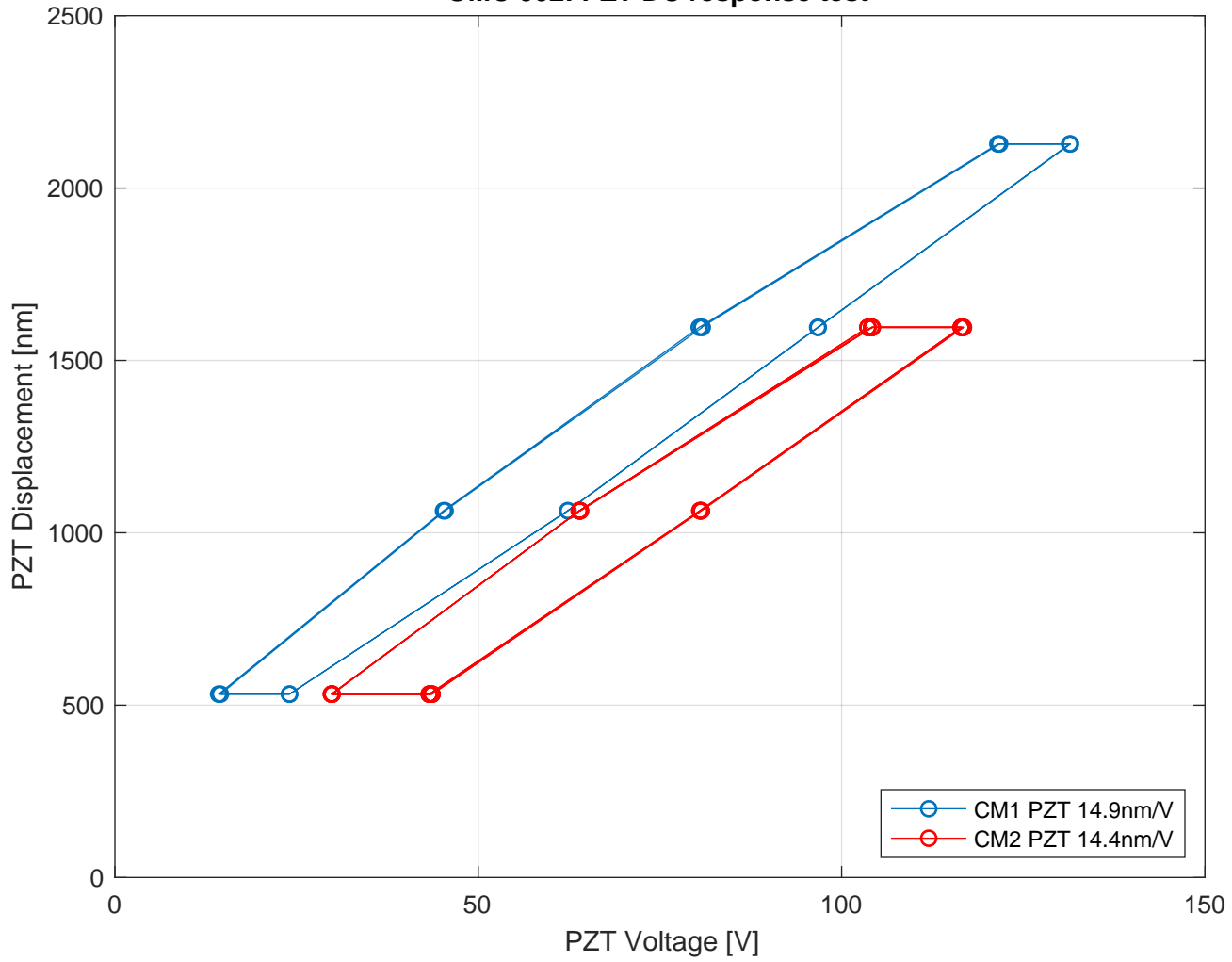
OMC 002: PZT DC response test
