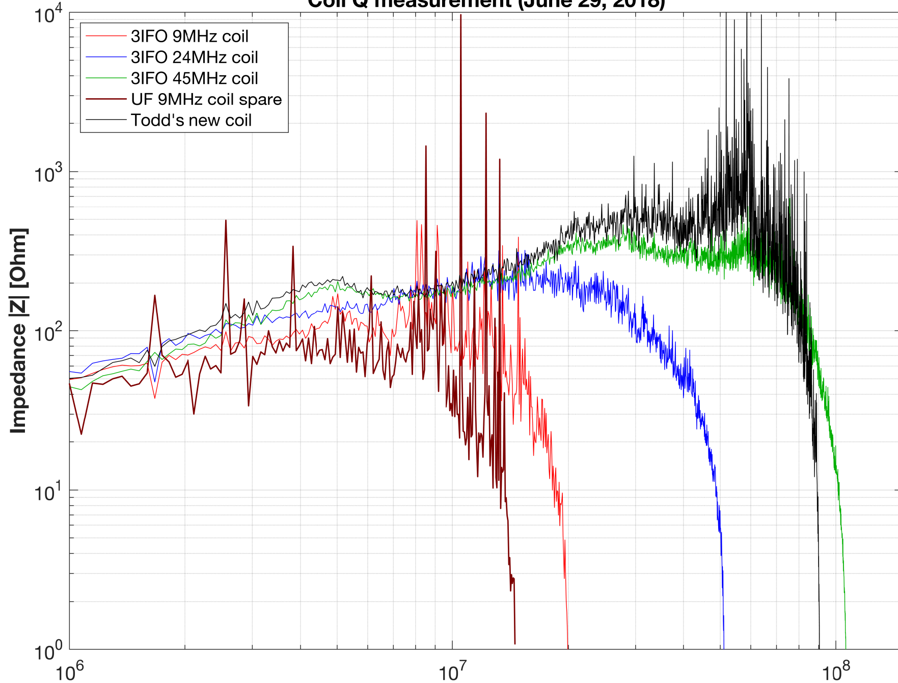
Coil Q measurement (June 29, 2018)
