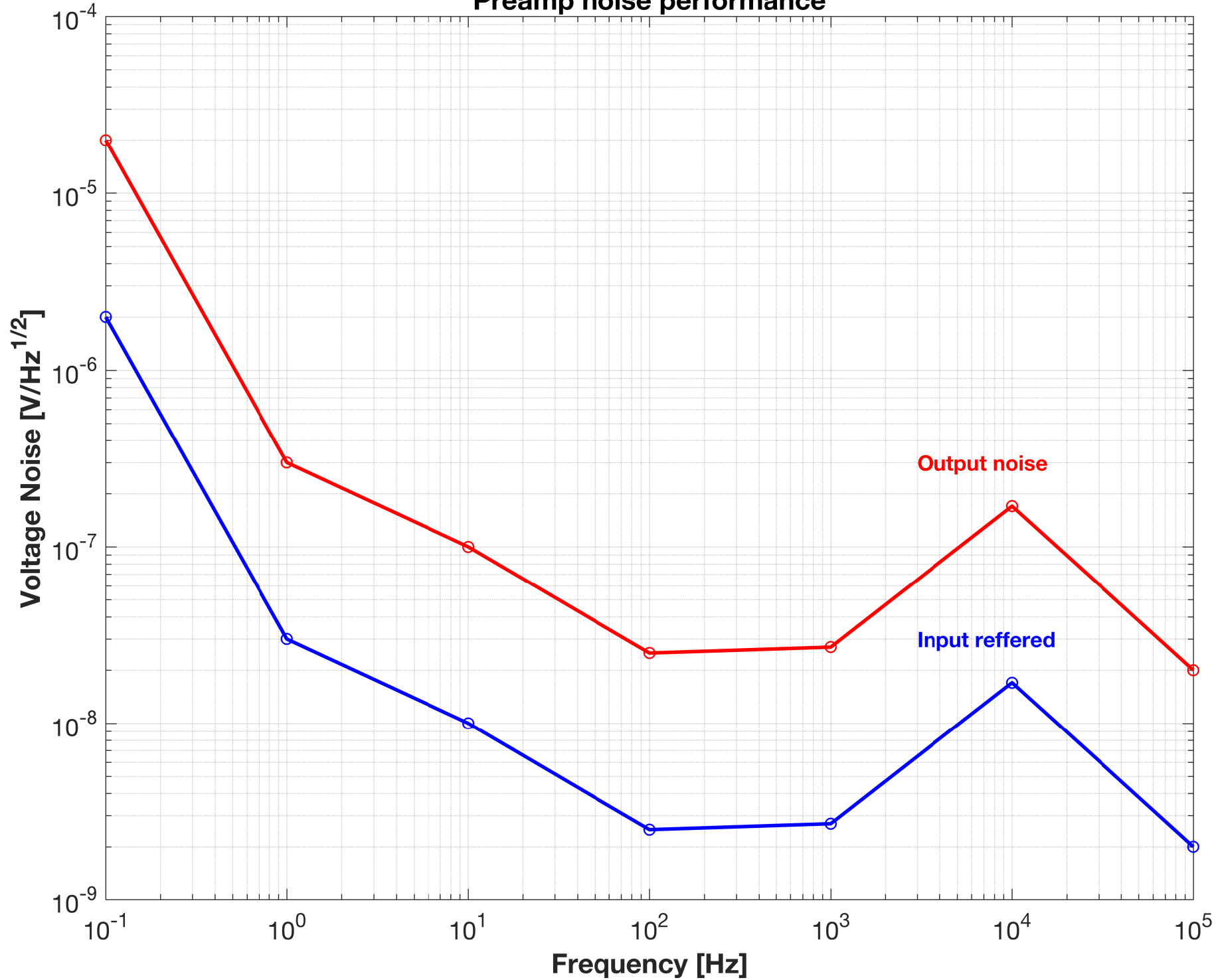
Preamp noise performance
