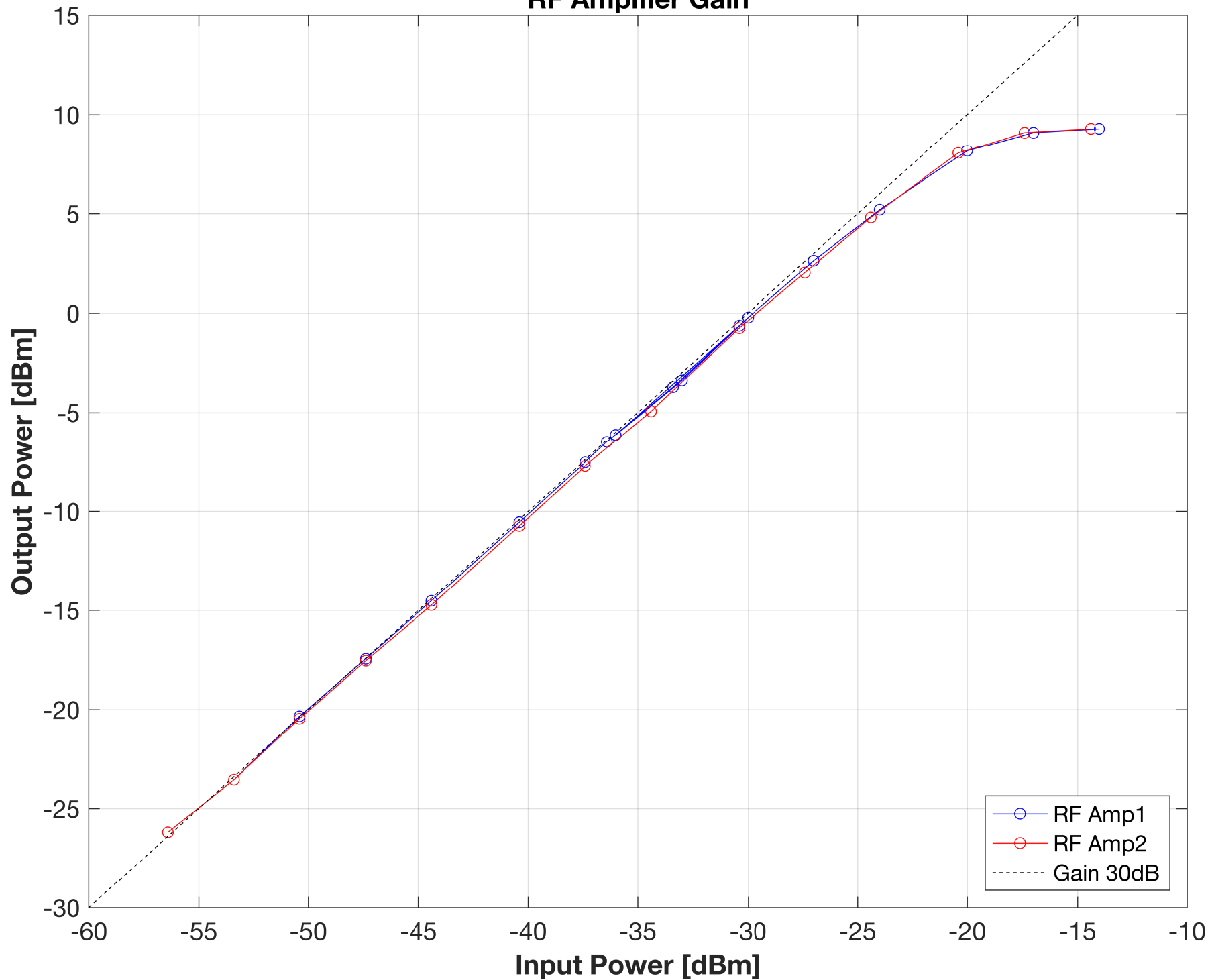
RF Amplifier Gain
