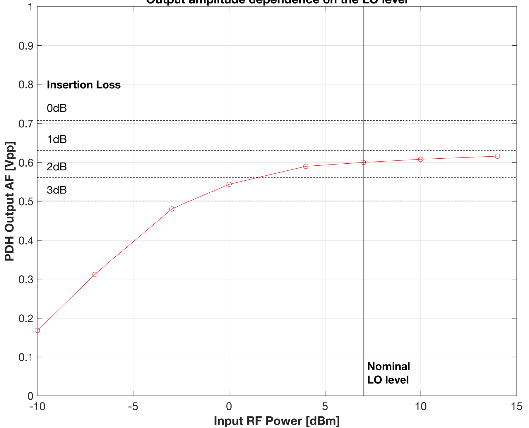
Output amplitude dependence on the LO level
