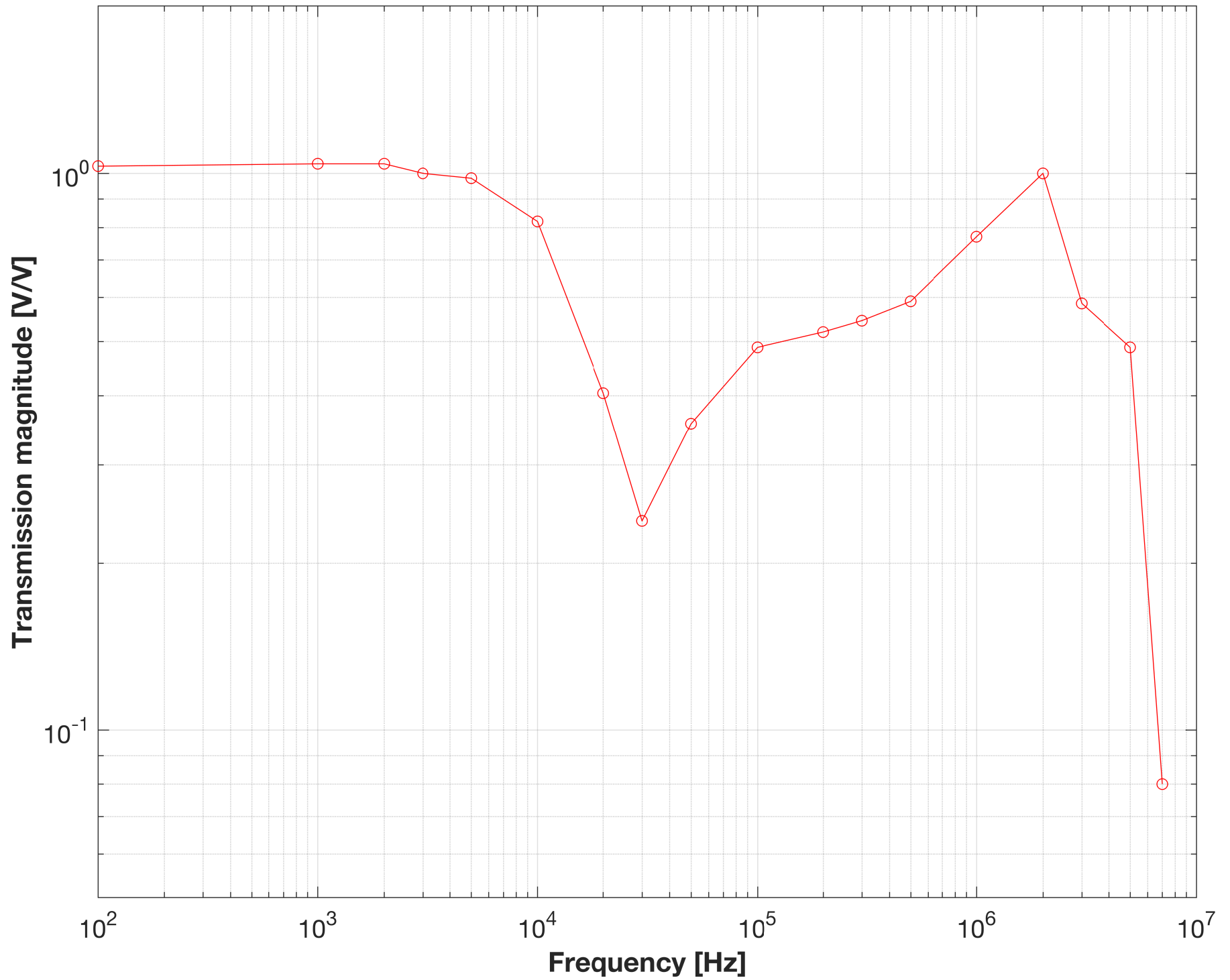
RF to AF transmission measurement
