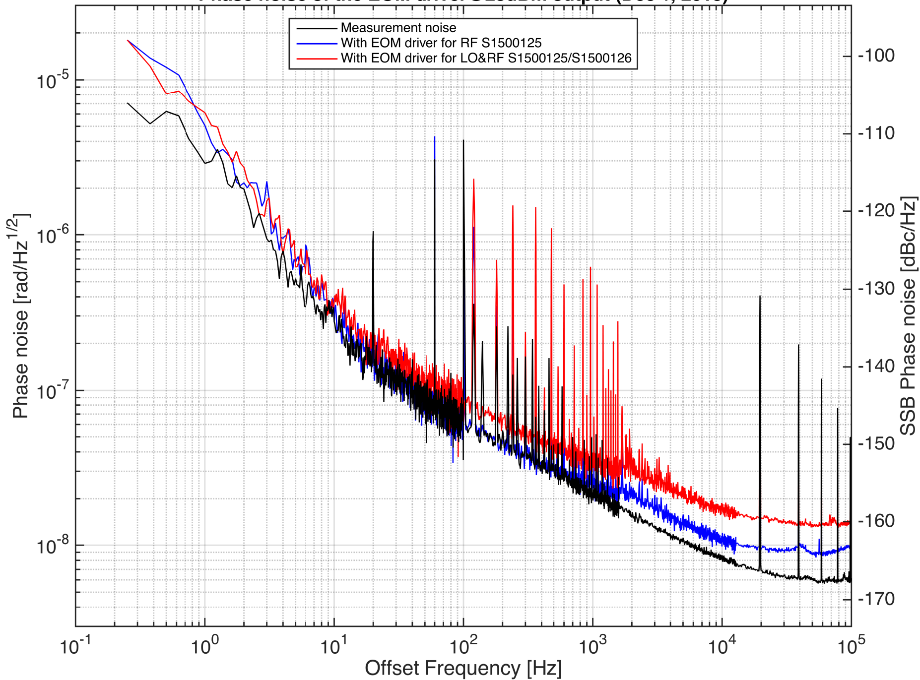
Phase noise of the EOM driver@23dBm output (Dec 1, 2015)
