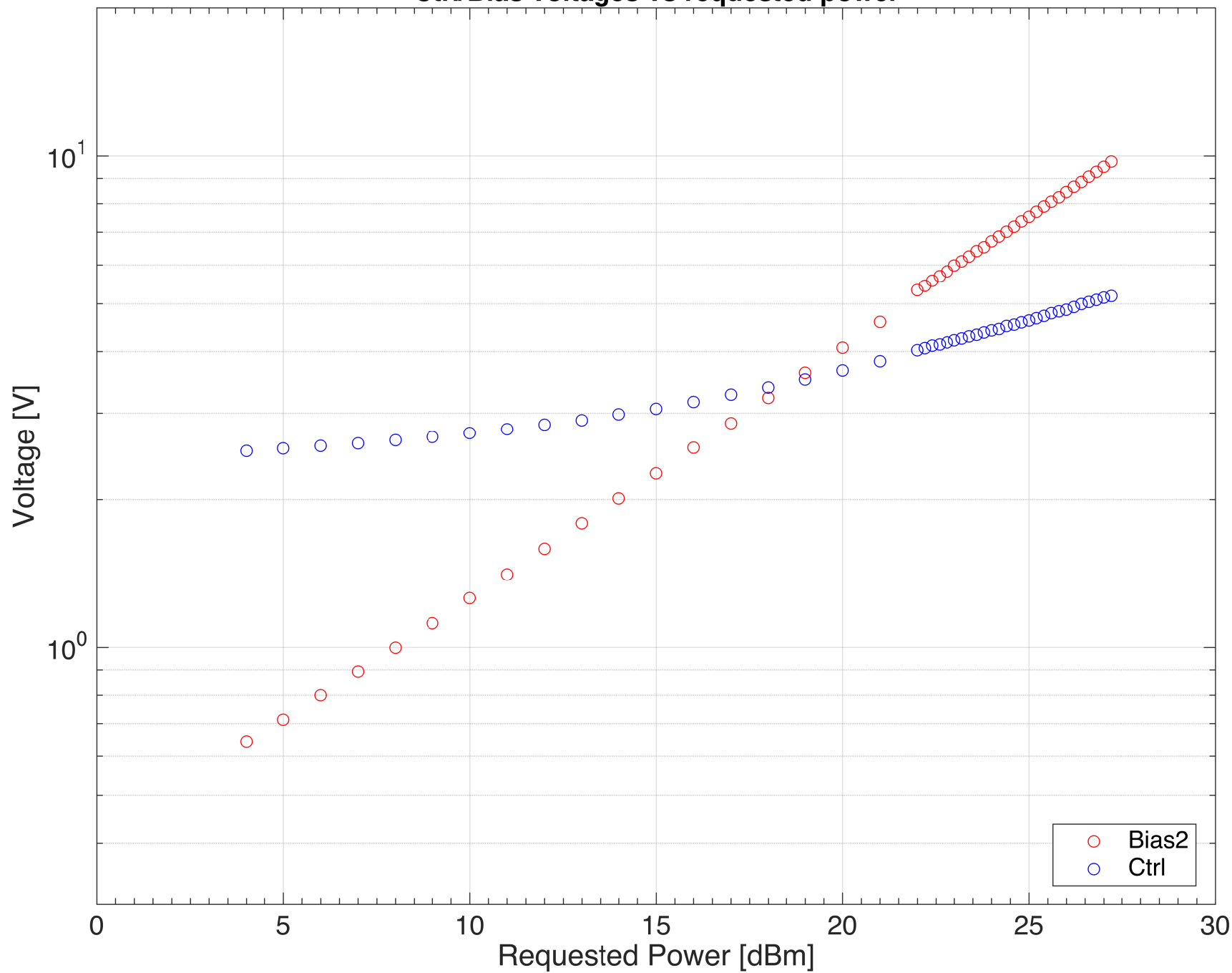
Ctrl/Bias voltages vs requested power
