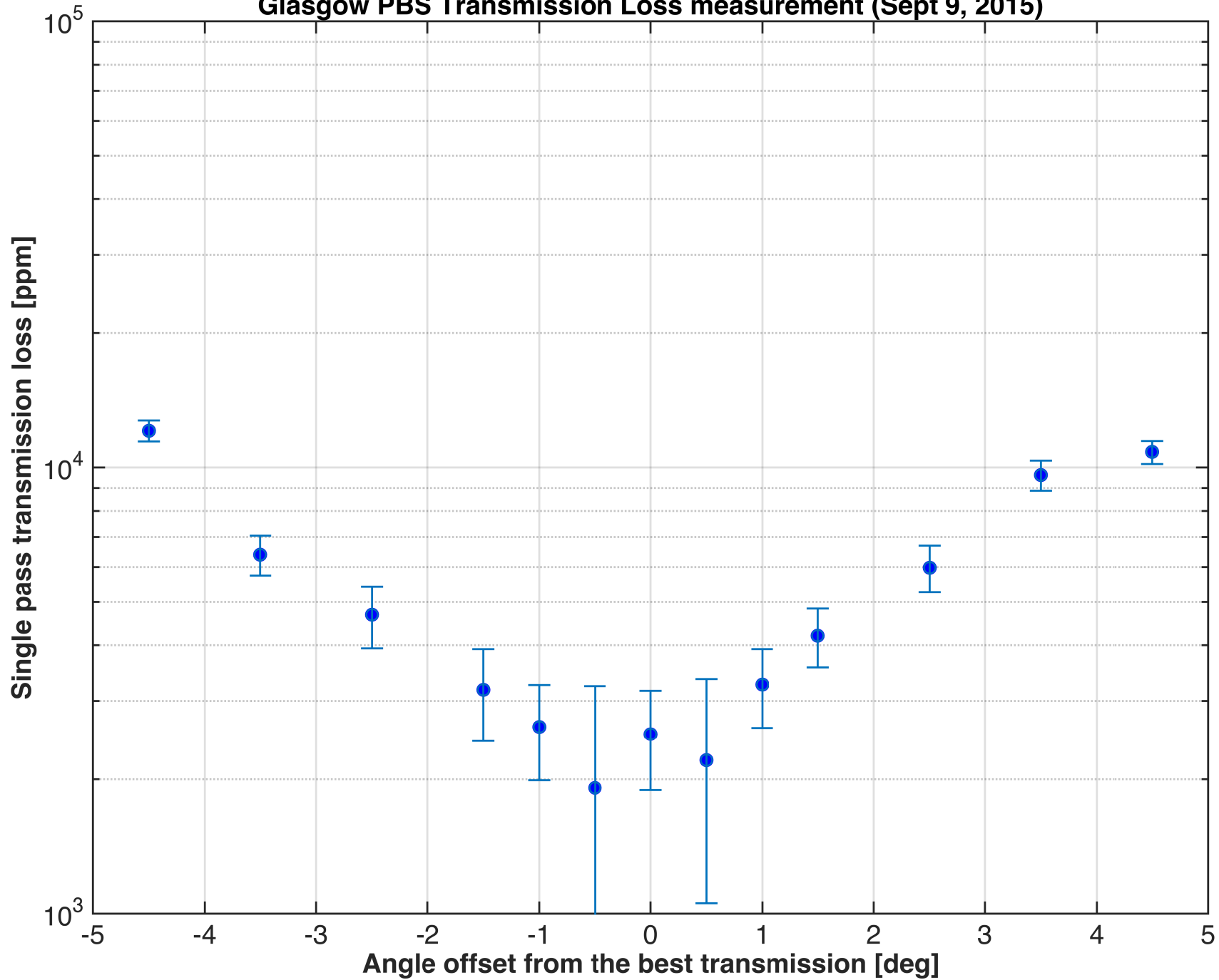
Glasgow PBS Transmission Loss measurement (Sept 9, 2015)
