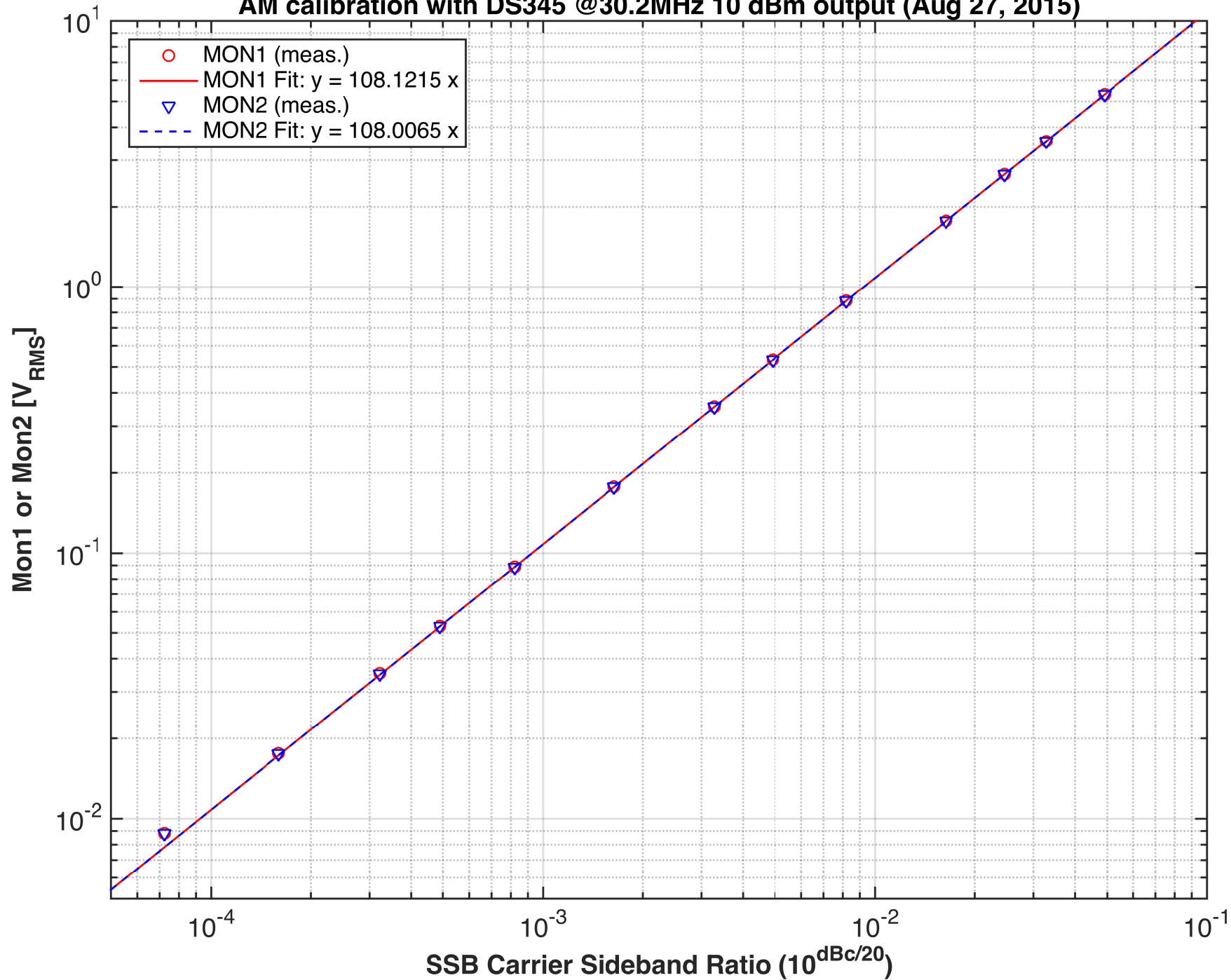
AM calibration with DS345 @30.2MHz 10 dBm output (Aug 27, 2015)
