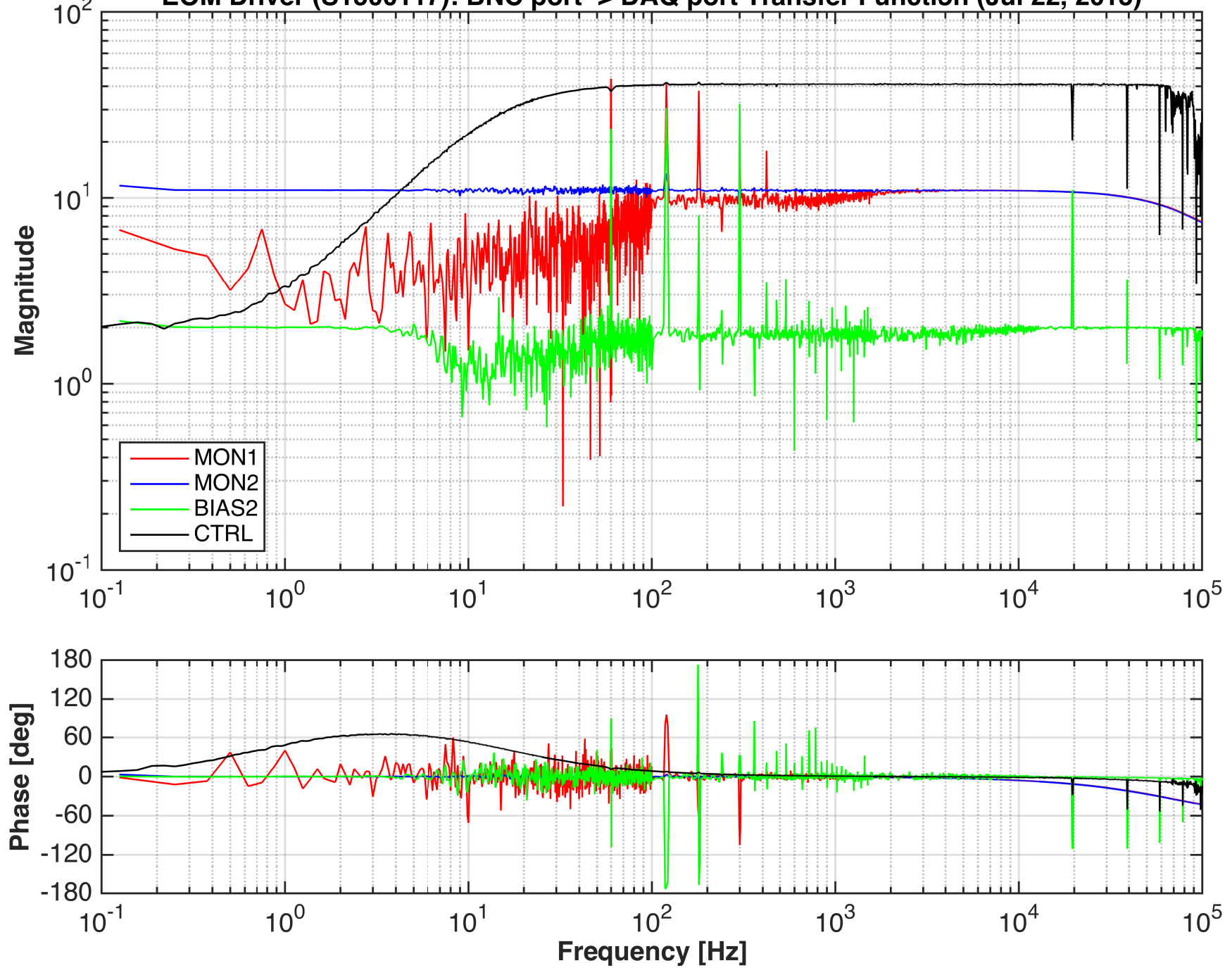
EOM Driver (S1500117): BNC port -> DAQ port Transfer Function (Jul 22, 2015)
