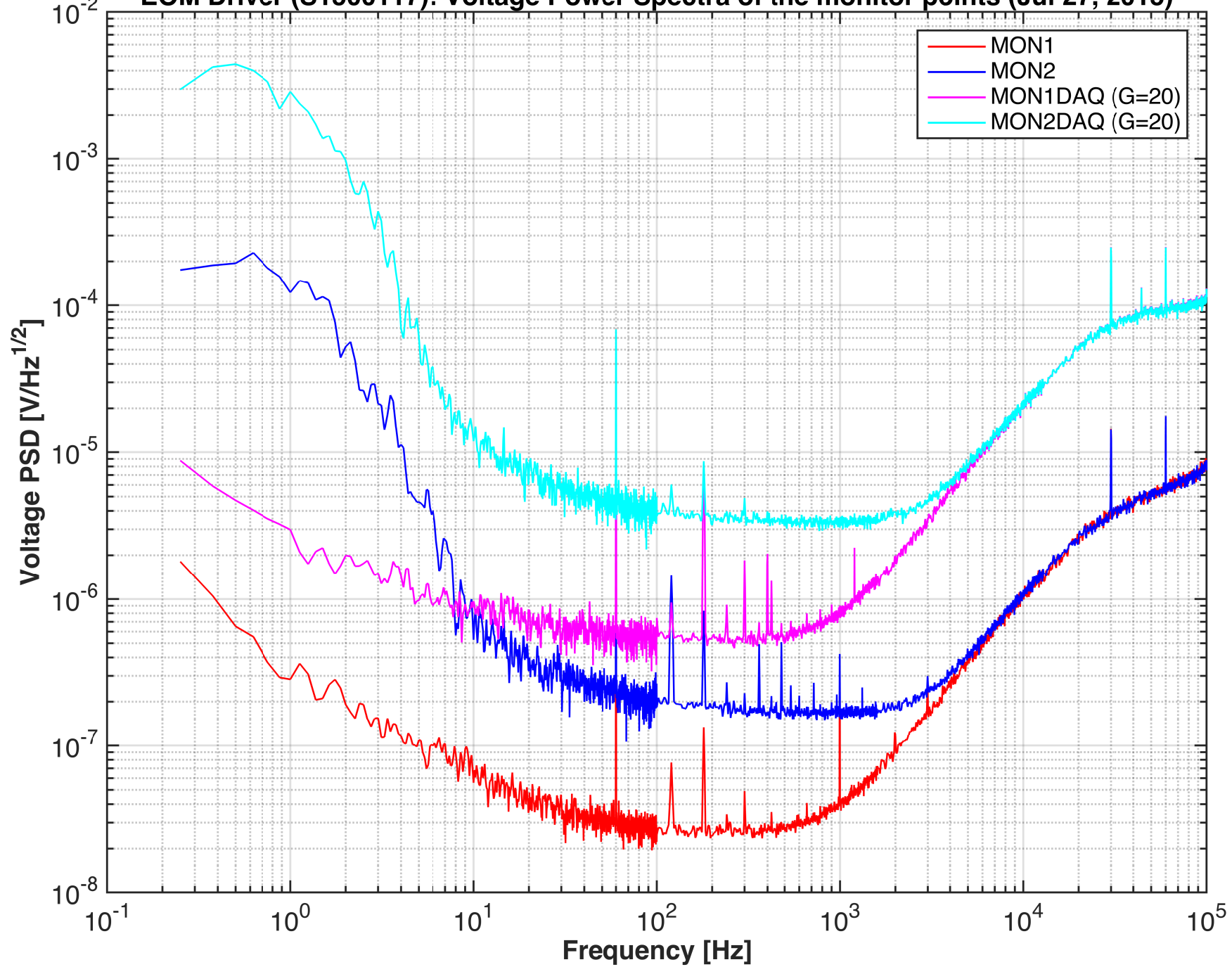
EOM Driver (S1500117): Voltage Power Spectra of the monitor points (Jul 27, 2015)
