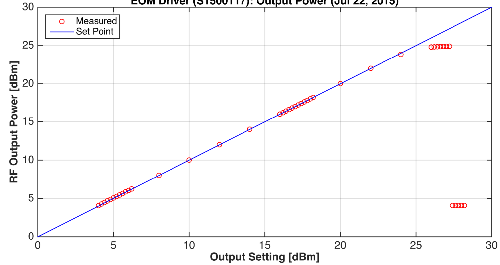
EOM Driver (S1500117): Output Power (Jul 22, 2015)
