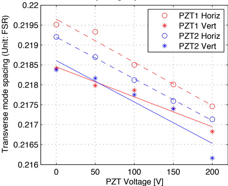
Transverse mode spacing dependence on the PZT voltage
